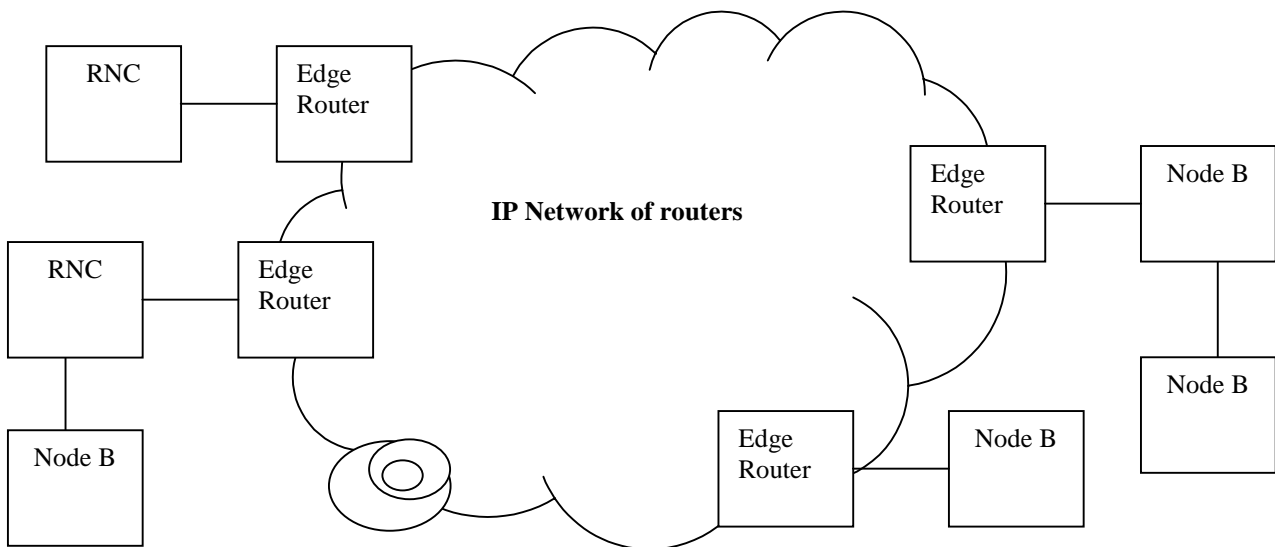
Figure 2921: Example Architecture for IP Transport Network
