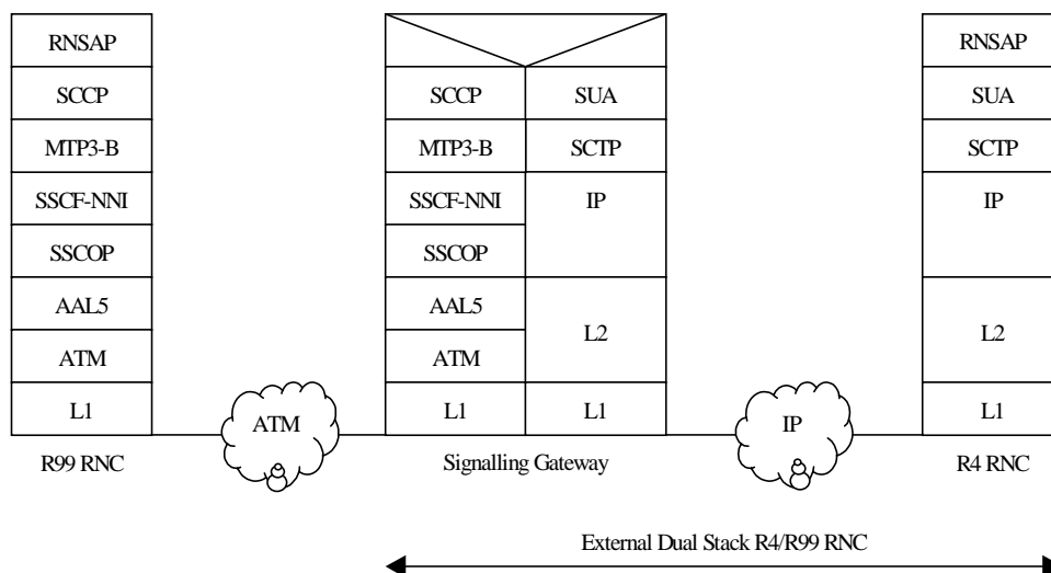
Figure 4837: Interworking between External dual stack RNC and a Rel4/R99 RNC.
