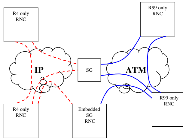
Figure 4938: Possible interworking scenarios using SUA.
