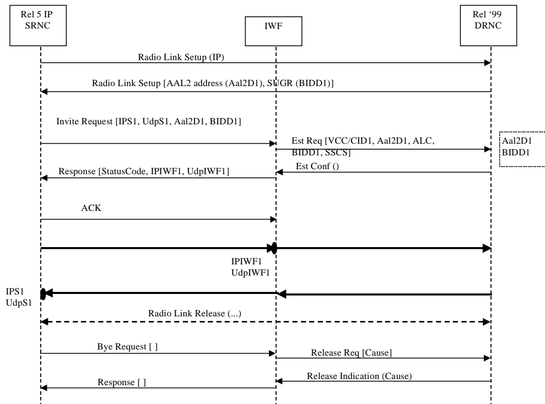
Figure 4433: Interworking between an AAL2/ATM SRNC and an IP DRNC
