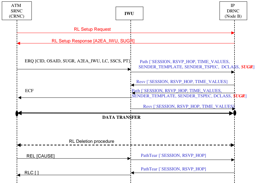
Figure 4736: Interaction between ATM SRNC (CRNC) and IP DRNC (Node B)
