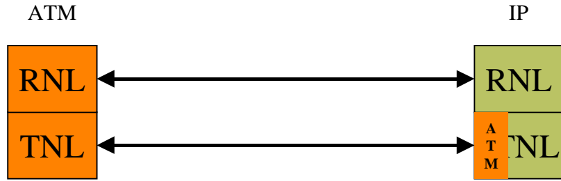
Figure 3223. Dual Stack operation within Rel.4 RNCs
