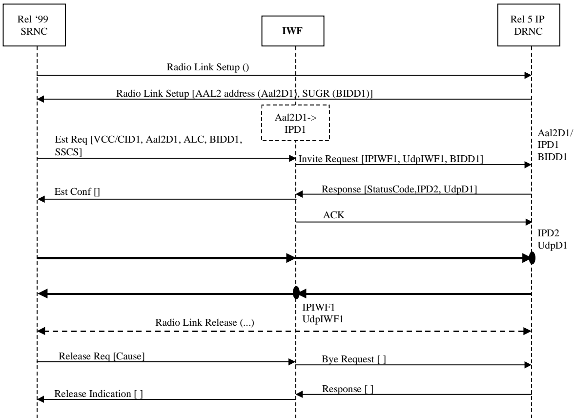
Figure 4332: Interworking between an AAL2/ATM SRNC and an IP DRNC
