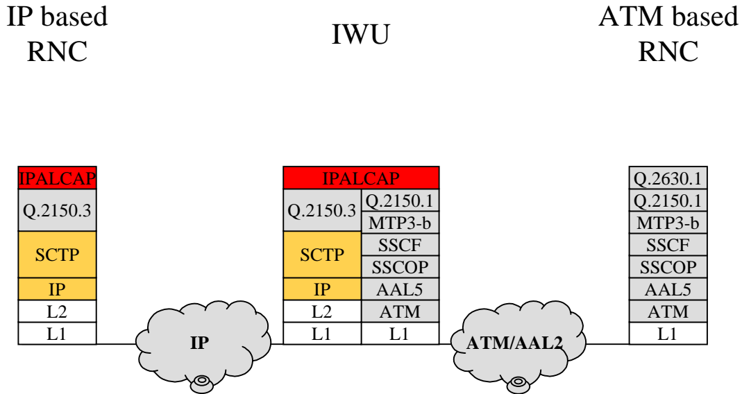
Figure 4534: Transport Network Control Plane Interworking
