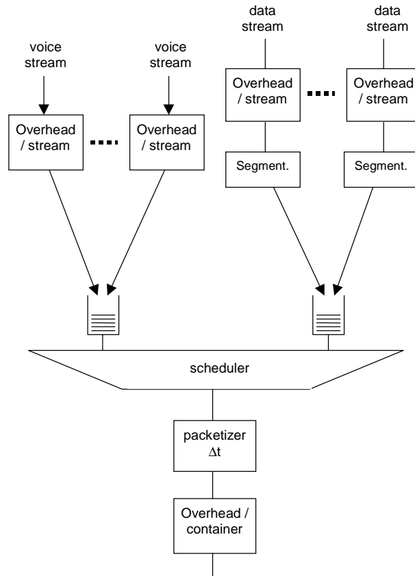
Figure 5342: Implementation Structure, Variant 2
