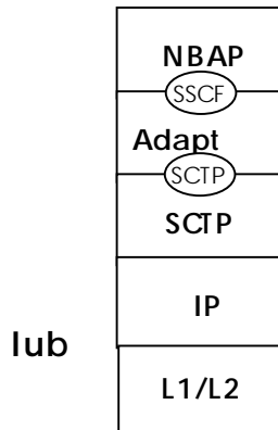
Figure 2618: Iub Signalling bearer protocol stack with Adaptation Layer
