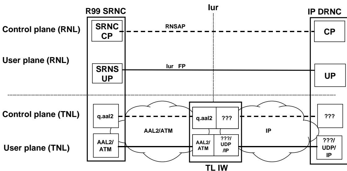
Figure 3928: Transport network layer interworking with release '99 SRNC
