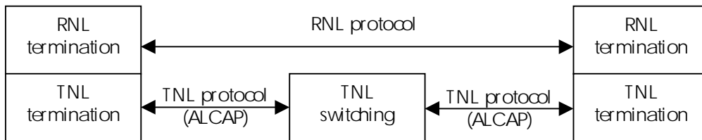
Figure 18 : RNL and TNL terminations
