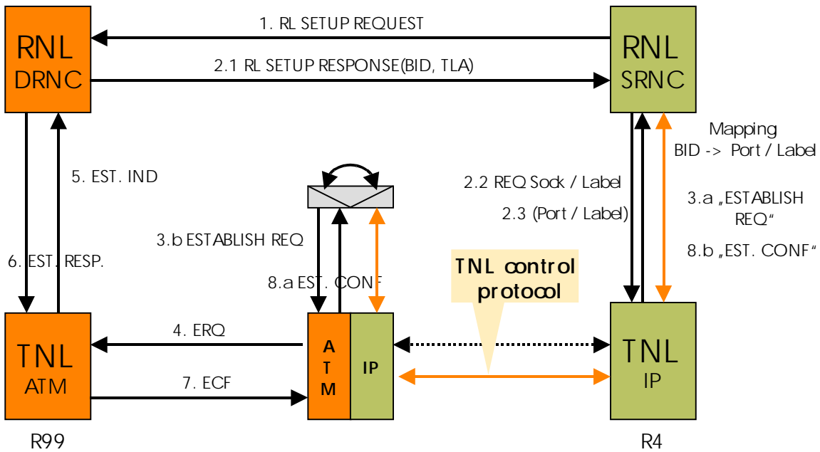
Figure 3727. Example 2: RNSAP: DCH RL Setup, DRNC = R99; SRNC = Rel.4
