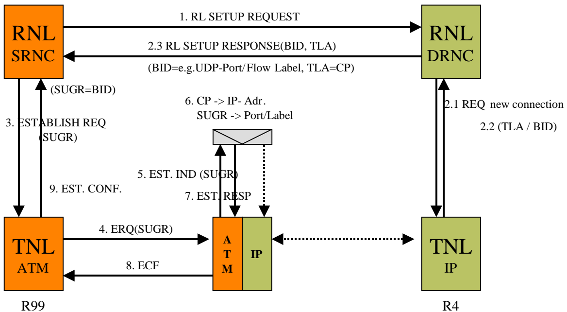
Figure 3526. Example 1: RNSAP: DCH RL Setup, SRNC = R99; DRNC = Rel.4
