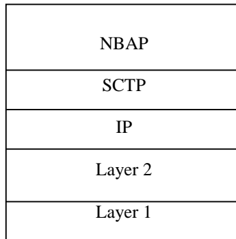
Figure 2517: Iub Signalling bearer protocol stack without Adaptation Layer
