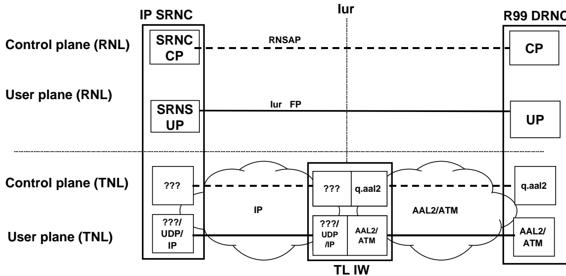
4029: Transport network layer interworking with IP SRNC
