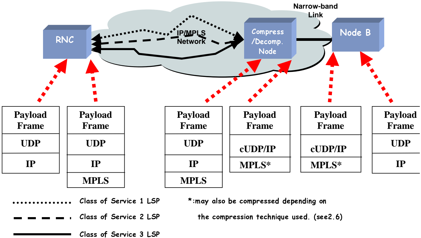
Figure 1411 Protocol stacks at key nodes in the network for a MPLS-based transport solution
