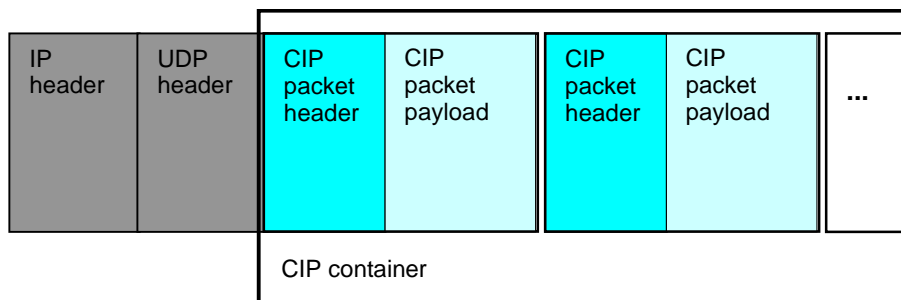
Figure 1: Generic CIP Container format
