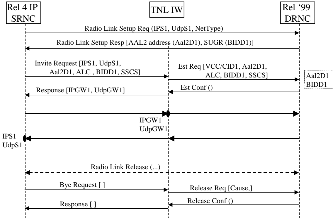
Figure 4231: Interworking between an AA2/ATM SRNC and an IP DRNC
