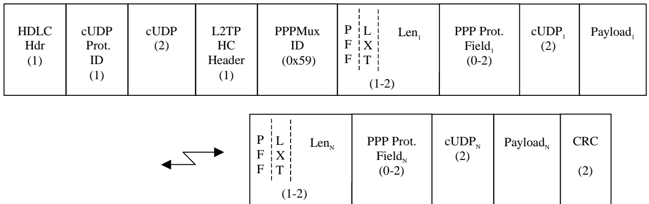
Figure 119: cTCRTTP PPPMux packet tunneled in L2TPHC over a PPP link
