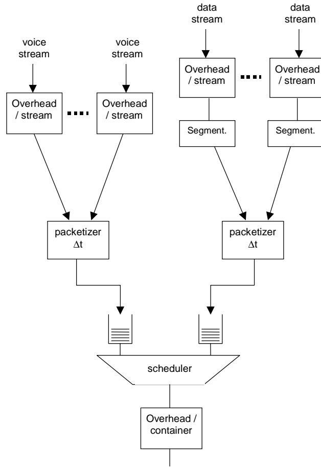
Figure 514: Implementation Structure, Variant 1
