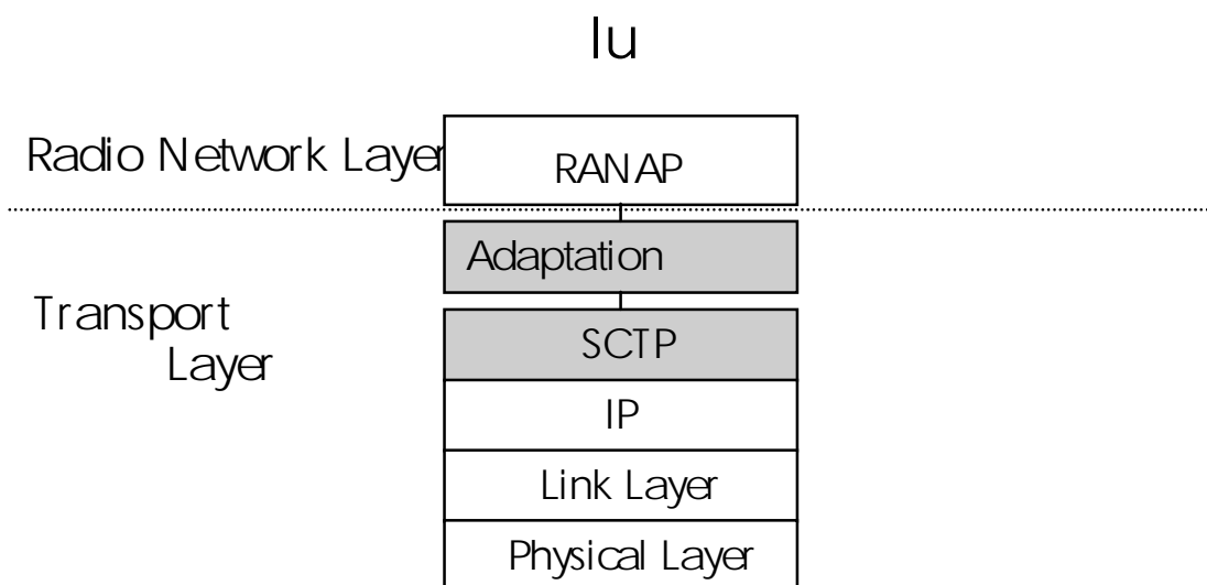
Figure 2719: RNL Signalling bearers on Iu interface, the principle.
