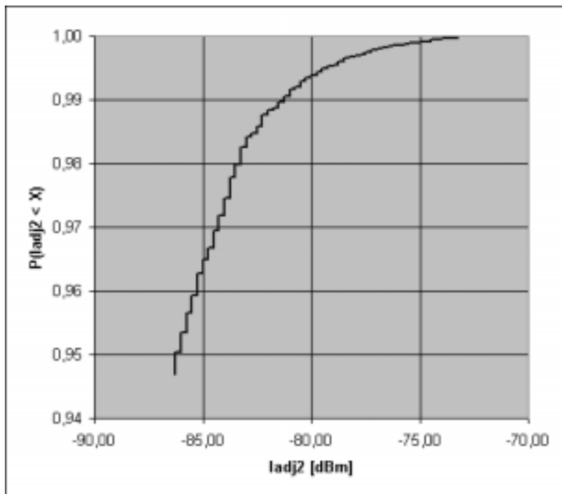
Figure 7.4: CDF of I_{adj2} originating from the second strongest interferer at the victim BS.
