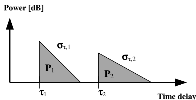
Figure 1. Channel shape (power delay profile) with multiple clusters.
