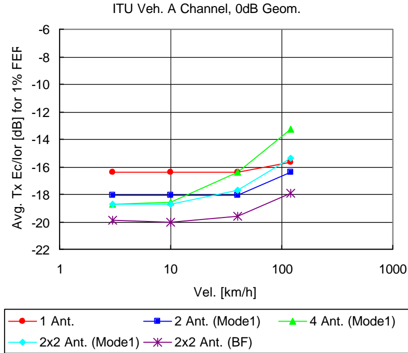
Figure 18. ITU Vehicular A channel, 0 dB geometry
