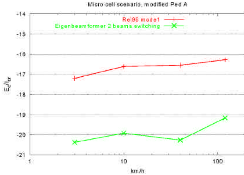
Figure 14. Simulation results for 0 dB geometry and micro cell scenario
