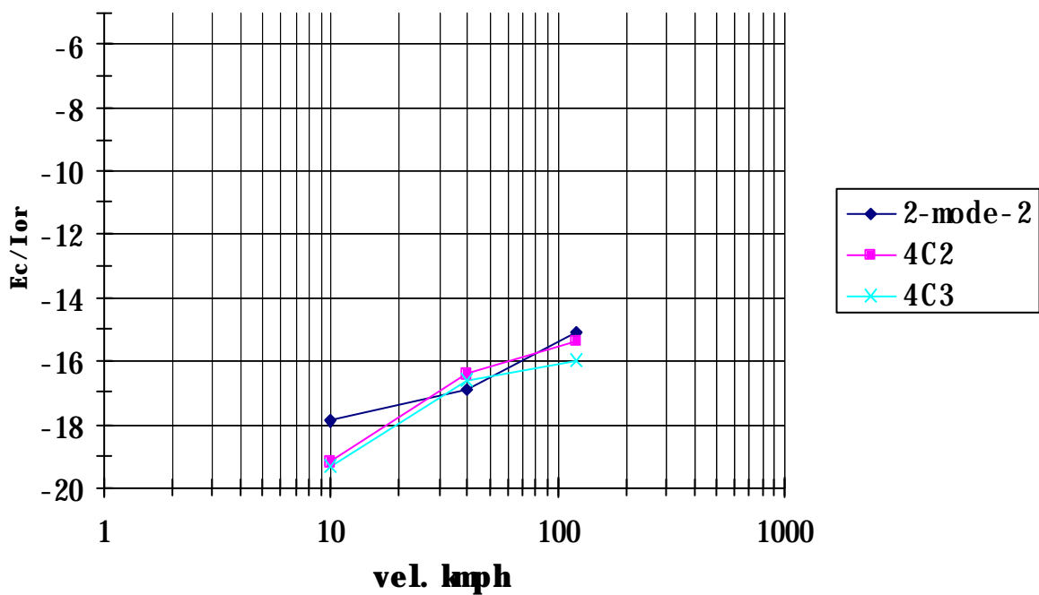
Figure 17. Simulation results for modified ITU Veh. A channel at 0 dB geometry.
