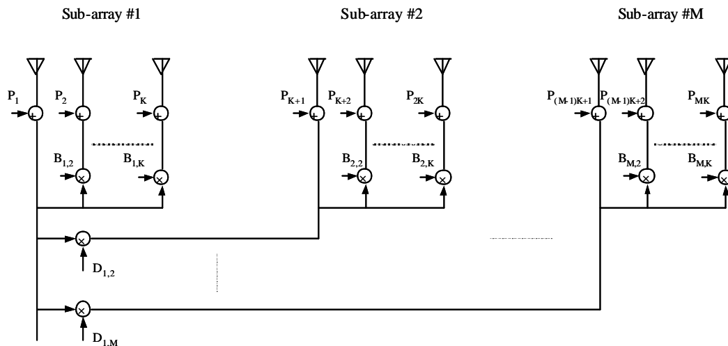
Figure 10. Hierarchical weighting for the transmit antenna diversity/beamforming
