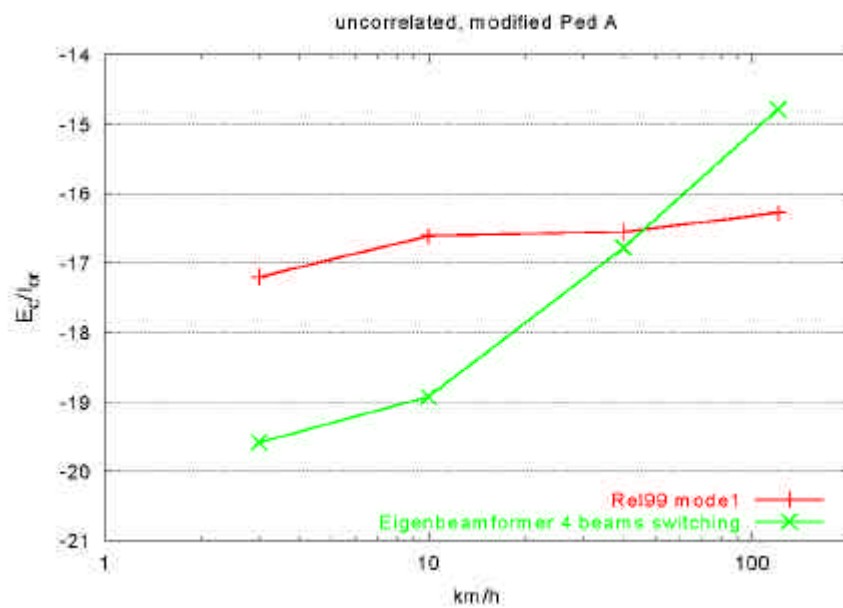
Figure 13. Simulation results for 0 dB geometry and uncorrelated antenna paths
