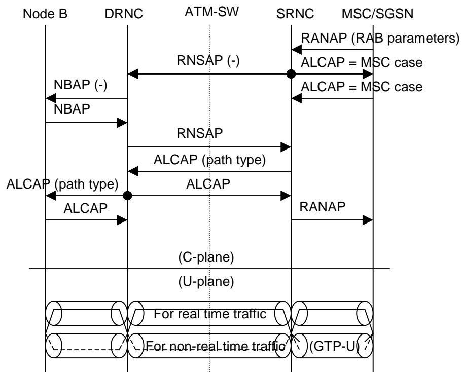
Figure 8: Direct and ATM switch cases
