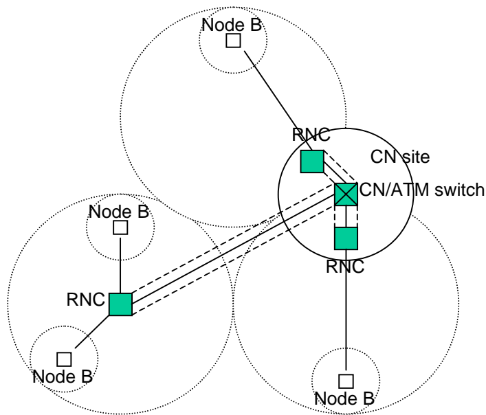
Figure 5: ATM switch
