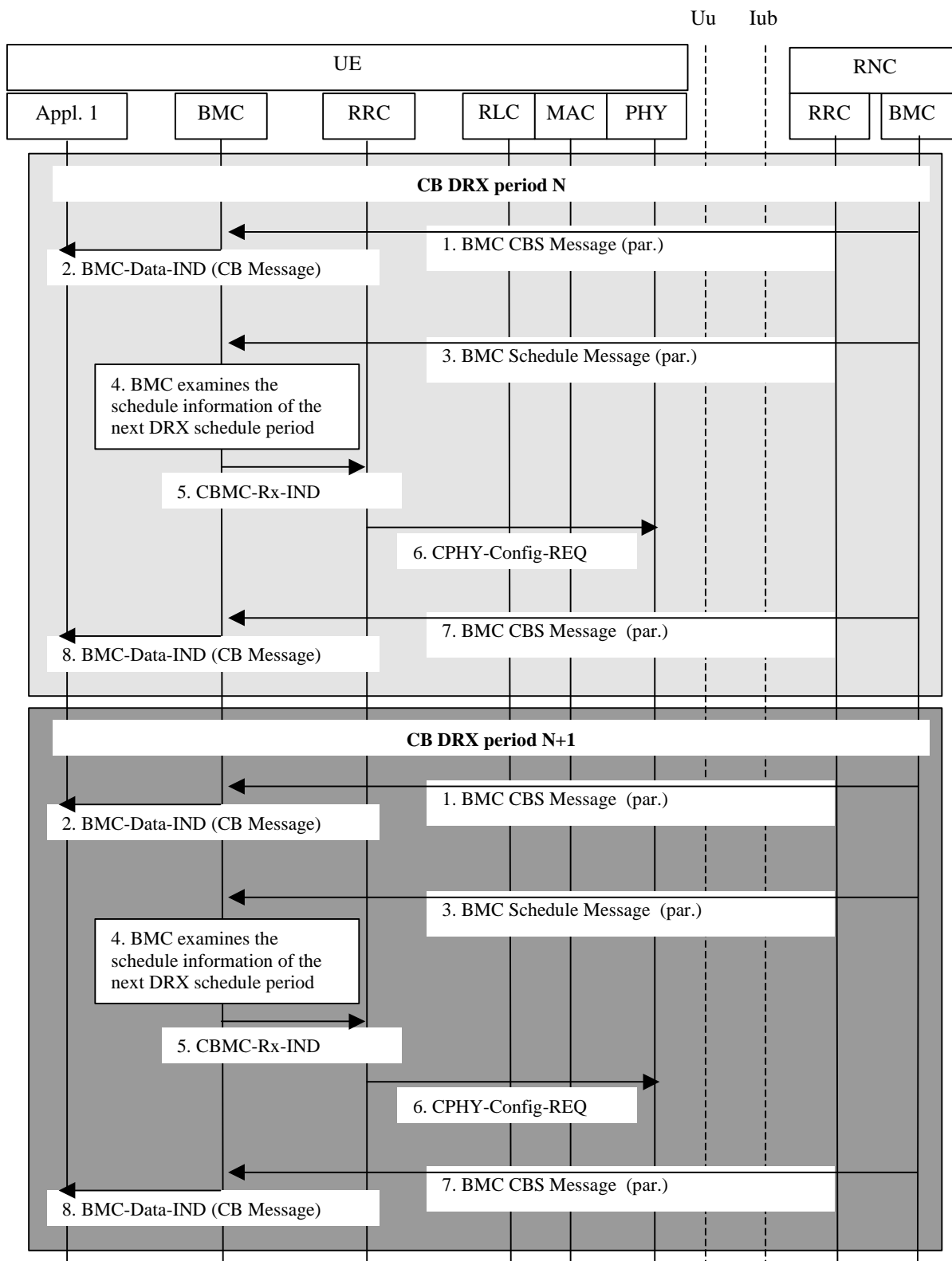
Figure 6.67: Example of Message Flow for CB message reception with DRX
