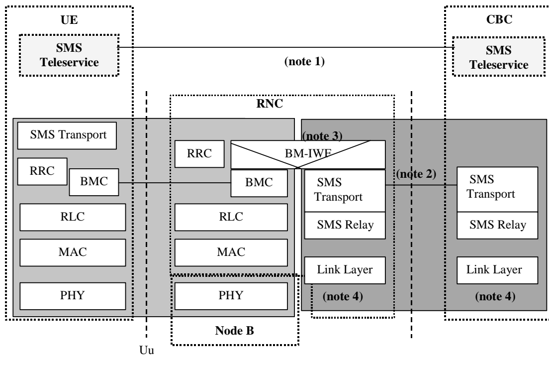
Figure 6.2: General Protocol Architecture when RNS is connected to ANSI-41 Core Network
