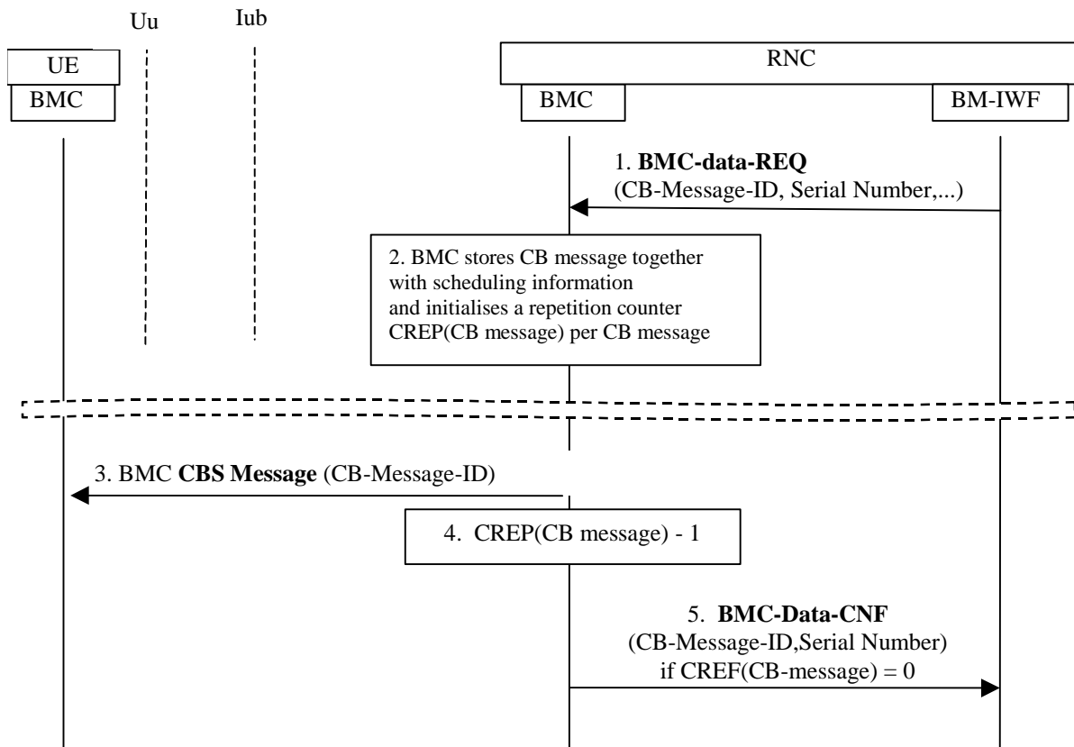
Figure 6.34: Example of Message Flow for broadcast of CBS related system information
