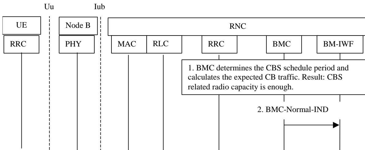
Figure 6.89: Example for Message Flow for Recovery from Overflow
