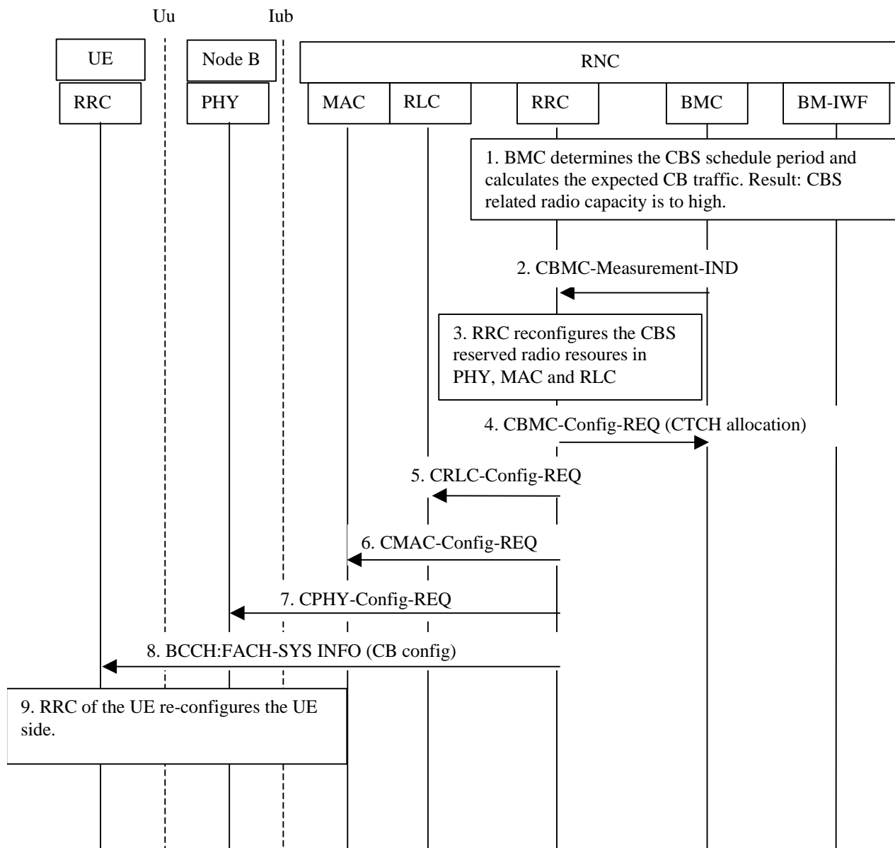
Figure 6.910: Example of Message Flow for Underflow
