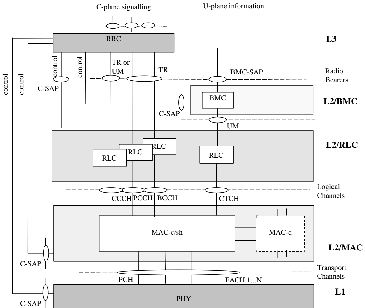
Figure 6.23: Protocol architecture on the radio interface
