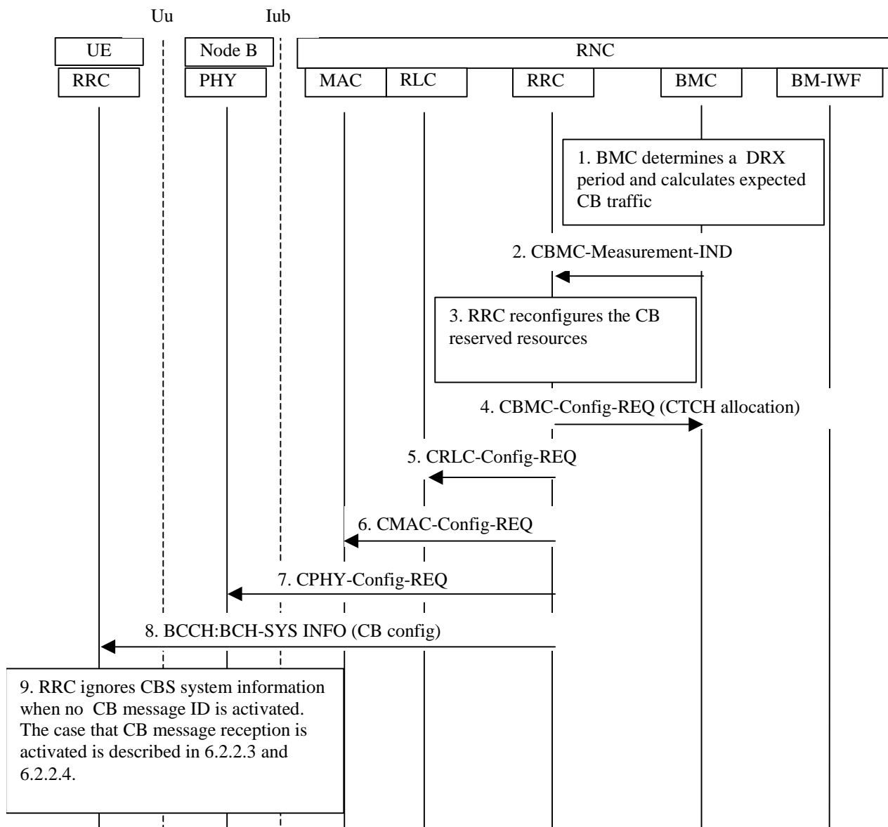
Figure 6.45: Example of Message Flow for BMC message scheduling
