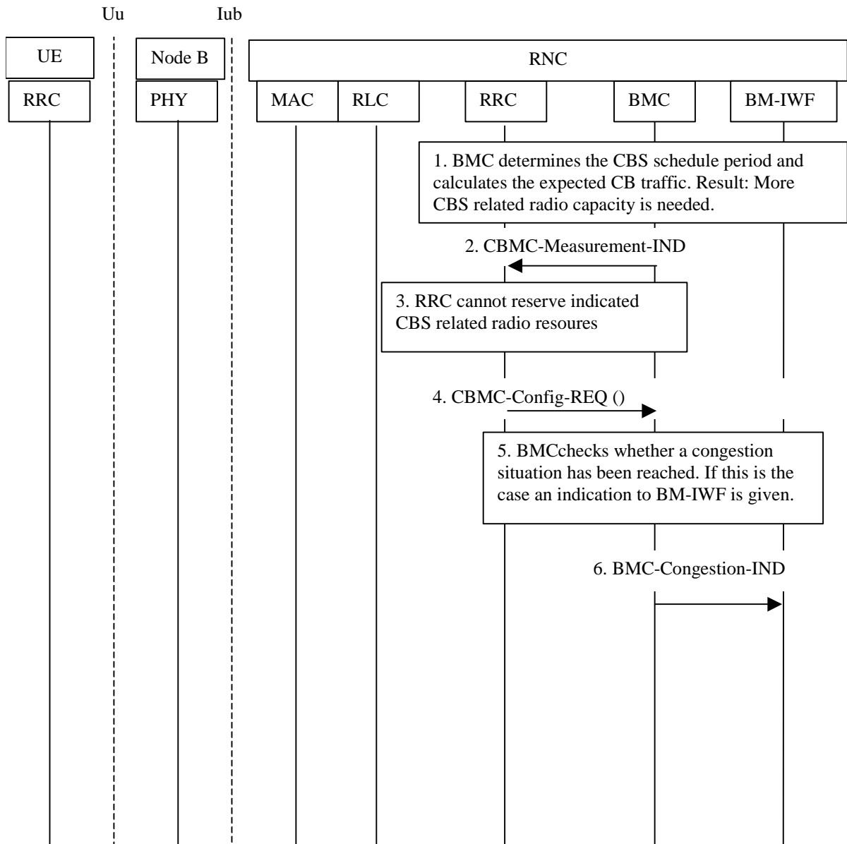
Figure 6.78: Example of Message Flow for Overflow
