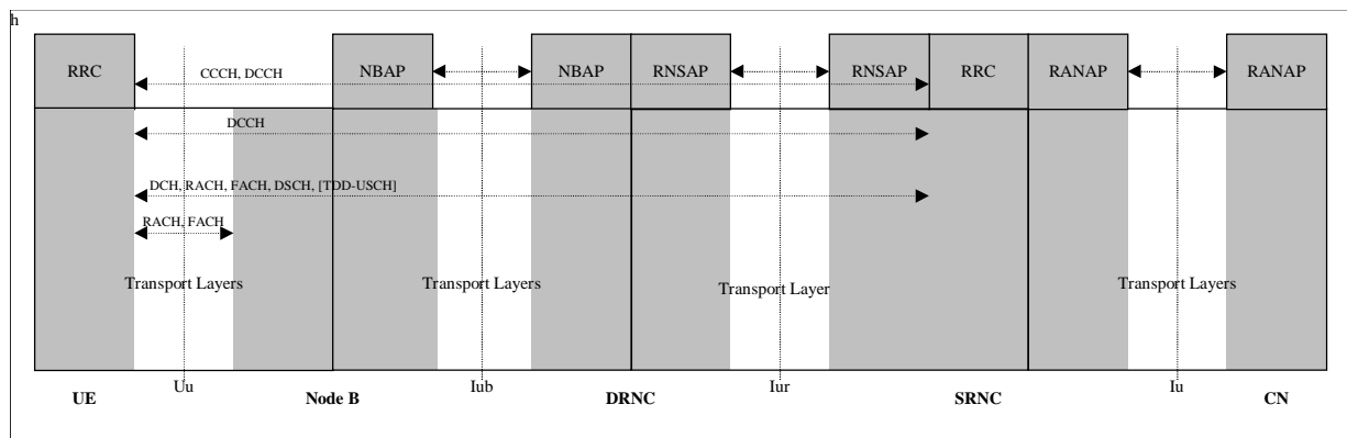
Figure 333: UTRAN and UE control plane protocol architecture (connected mode)
