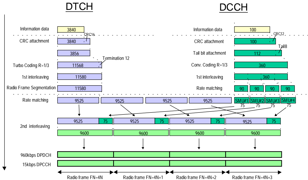
Figure A.x (Informative): Channel coding of UL reference measurement channel (384 kbps)
