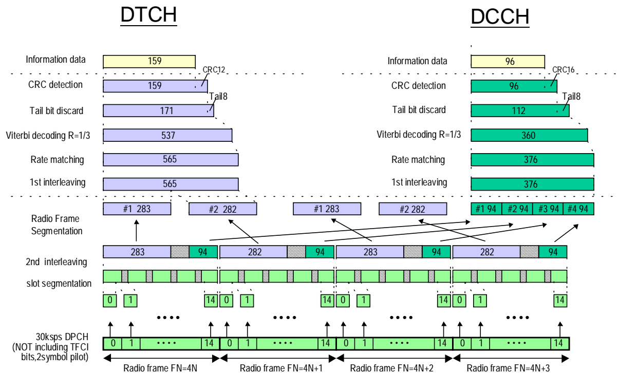
Figure A.10(Informative): Channel coding of DL reference measurement channel for BTFD (Rate 2)
