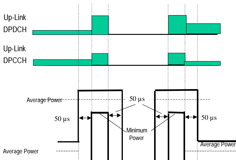
Figure 2 Transmit template during Compressed mode.
