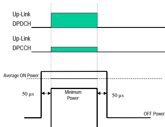
Figure 1a: Transmit ON/OFF template
