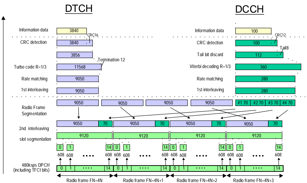
Figure A.x (Informative): Channel coding of DL reference measurement channel (384 kbps)
