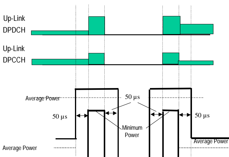
Figure 6.3 Transmit template during Compressed mode.
