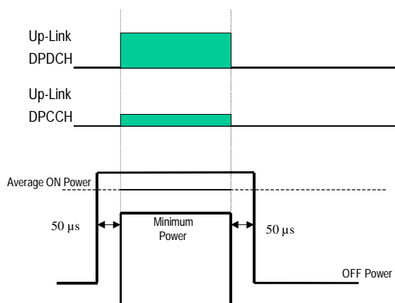
Figure 6.1: Transmit ON/OFF template
