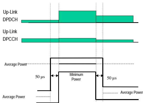
Figure 1b Transmit template during TFC change
