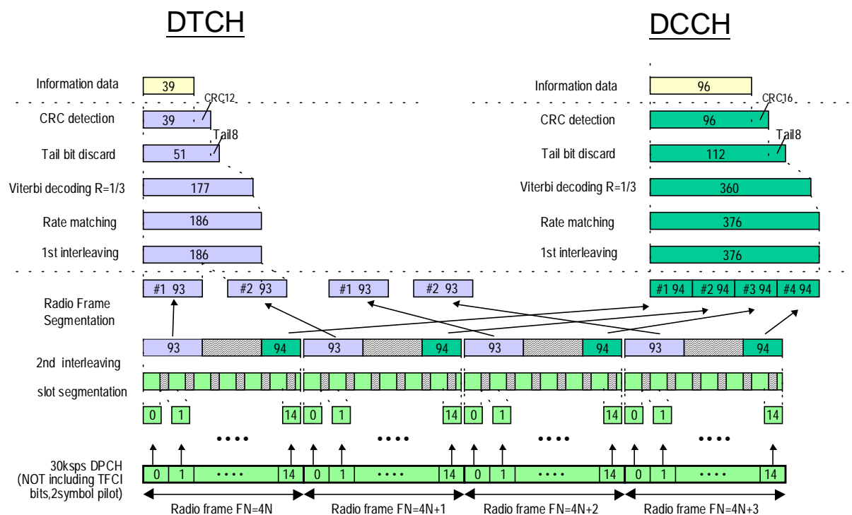
Figure A.11(Informative): Channel coding of DL reference measurement channel for BTFD (Rate 3)
