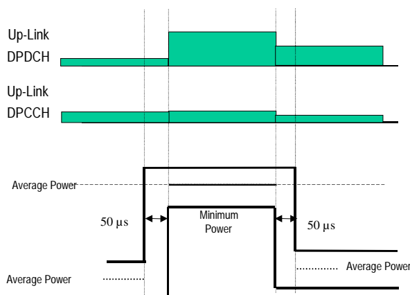
Figure 6.2 Transmit template during TFC change
