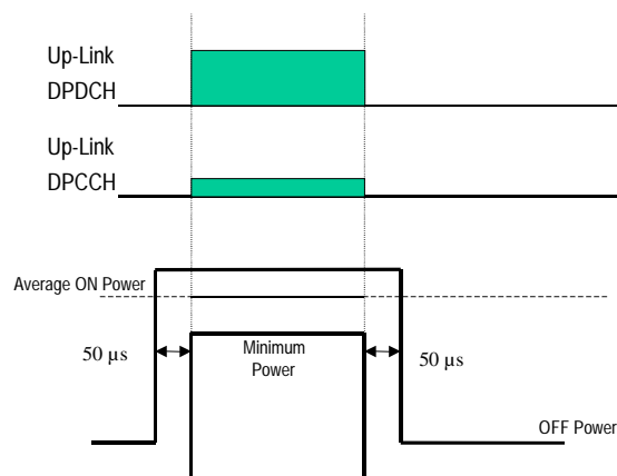
Figure 1a: Transmit ON/OFF template
