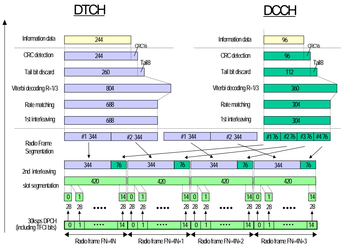
Figure A.5 (Informative): Channel coding of DL reference measurement channel (12.2 kbps)
