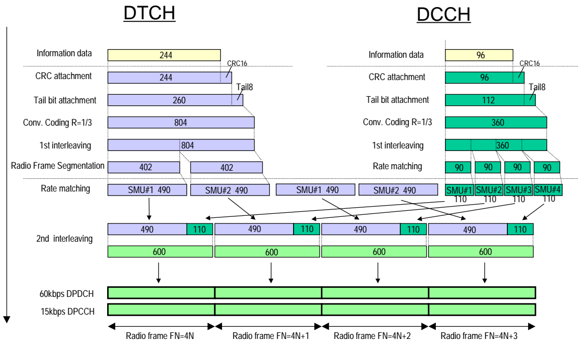
Figure A.1(Informative): Channel coding of UL reference measurement channel (12.2 kbps)
