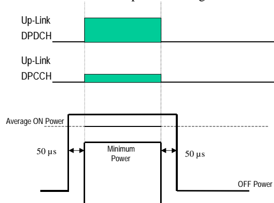
Figure 1a: Transmit ON/OFF template
