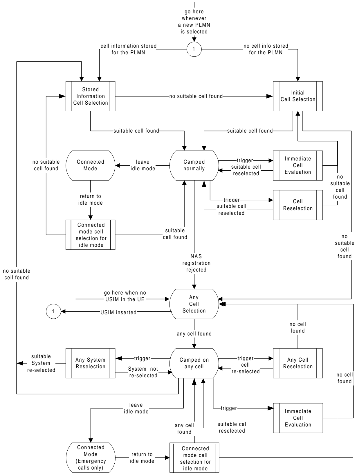
Figure 2: Idle Mode Cell Selection and Reselection
