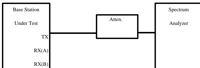
Fig. 6.6-1 6.6-16.6-1 Functional Setup for Transmission on/off Ratio Test.
