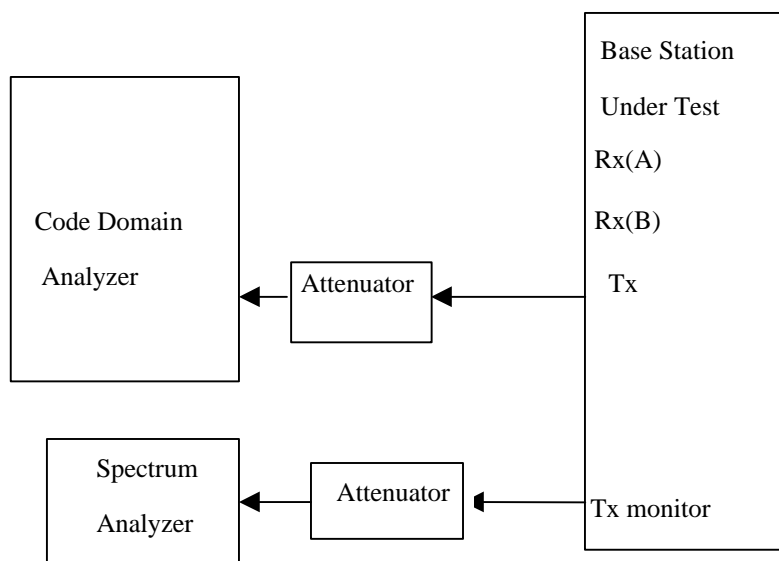
Fig. 6.5-136.5-96.5-5 Configuration for measurement
