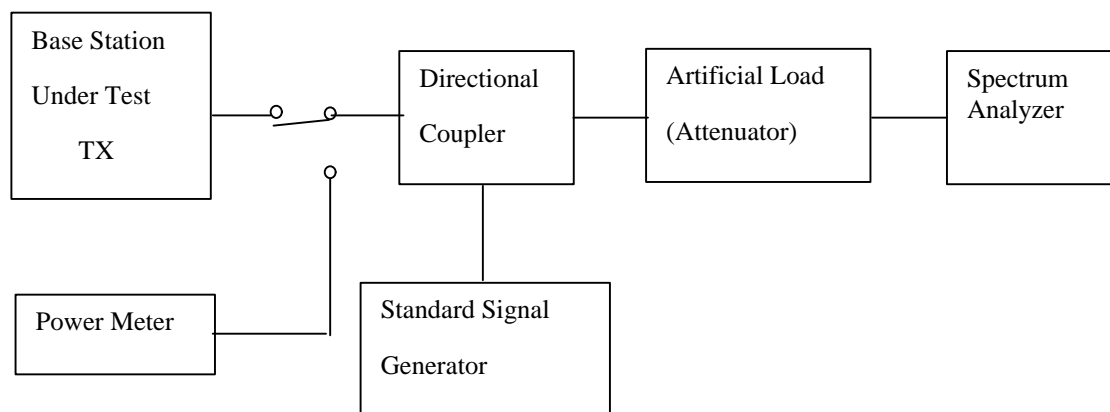
Fig. 6.8-16.8-16.8-1 Functional Setup for Base Station Intermodulation Spurious Response Testes
