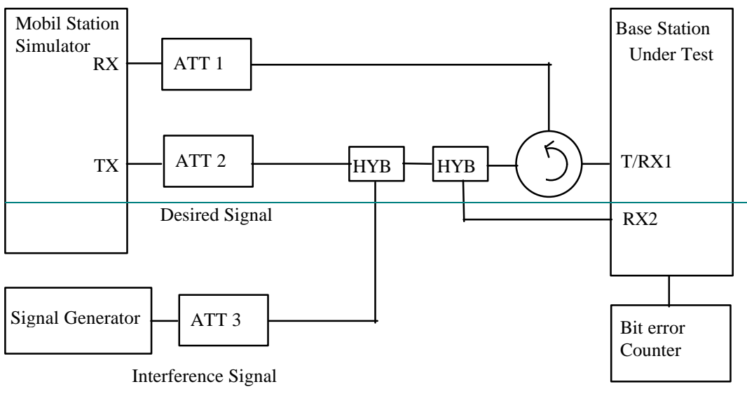
Fig. 7.6-1 Measuring system Setup for Spurious Response
