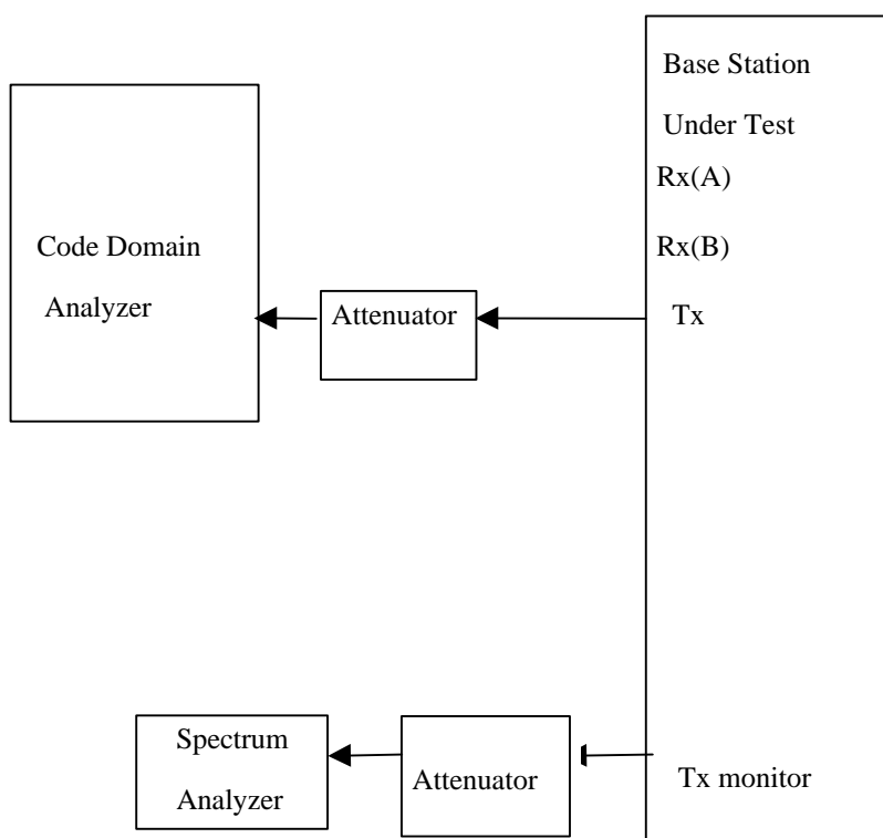
Fig. 6.5-76.5-56.5-3 Configuration for measurement
