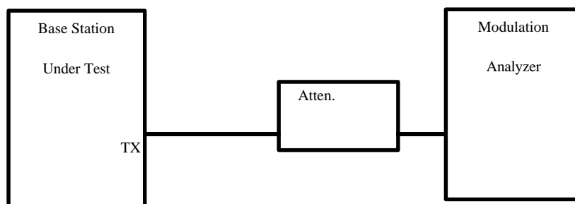
Fig. 6.9- 16.9-16.9-1 Functional Setup for Modulation Accuracy Test.
