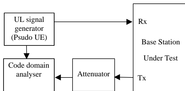
Fig. 6.5-16.5-16.5-1 Configuration for power control steps measurement
