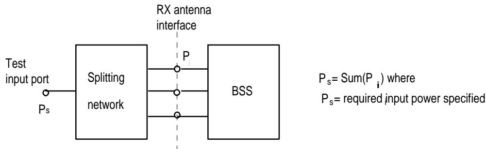
Fig. 4.13-1 Receiver test setup
