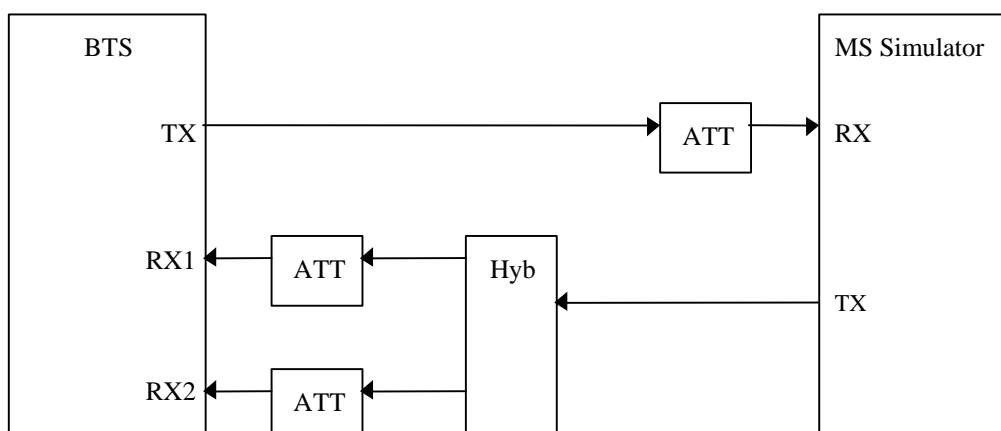
Fig. 7.2-1 7.2-1 Functional Setup for Base Station Reference sensitivity level Testes ( without duplex operation case )
