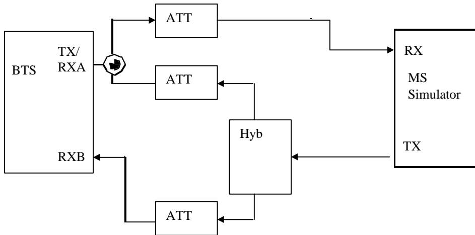
Fig. 7.2- 37.2-27.2-2 Functional Setup for Base Station Reference Sensitivity level Testes ( with duplexing operation case )
