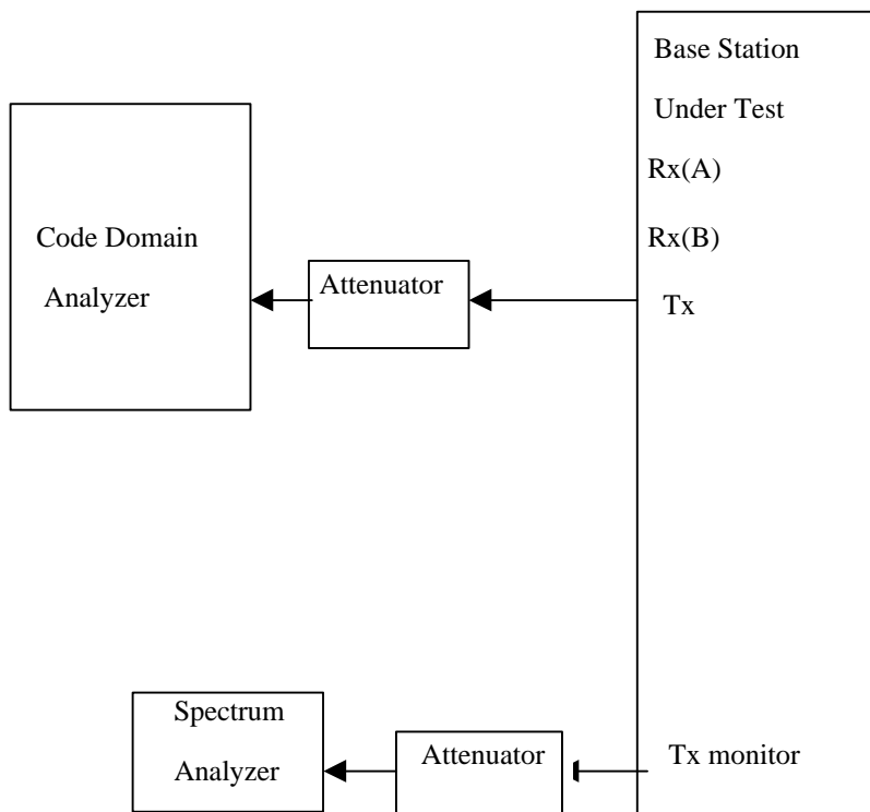
Fig. 6.5-46.5-36.5-2 Configuration for measurement
