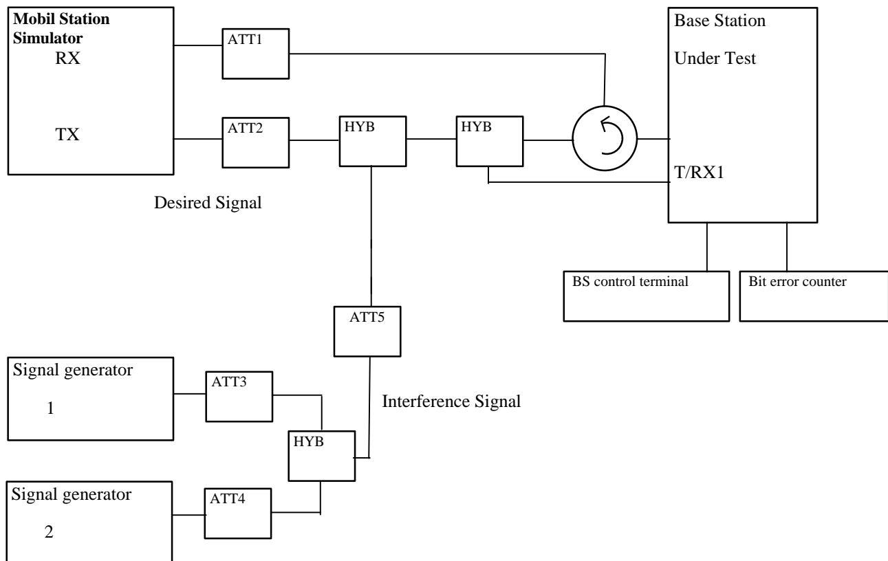
Fig. 7.6-17.8-17.8-1 Measuring system Setup for Reception Intermodulation sensitivity
