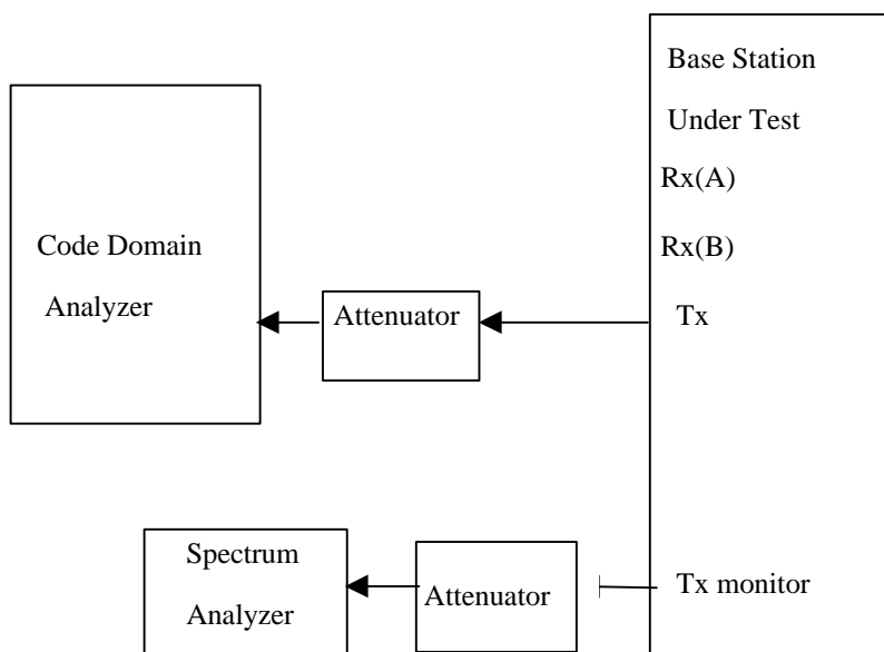
Fig. 6.5-106.5-76.5-4 Configuration for measurement
