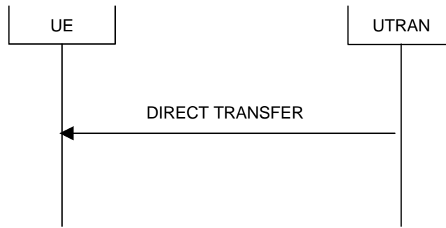
Figure 1643. Direct transfer in the downlink, normal flow
