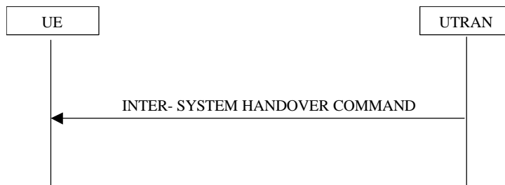
Figure 4542. Inter system handover from UTRAN, successful case
