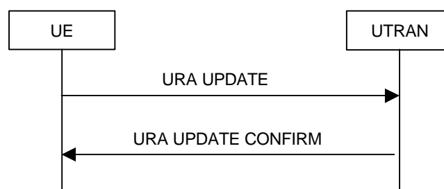
Figure 3734. URA update procedure, basic flow
