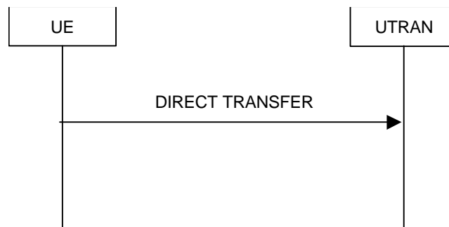
Figure 1744. Direct transfer in the uplink, normal flow
