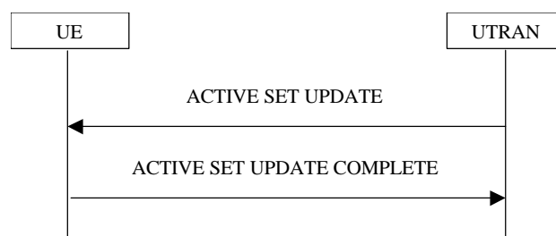
Figure 4037. Active Set Update procedure, successful case
