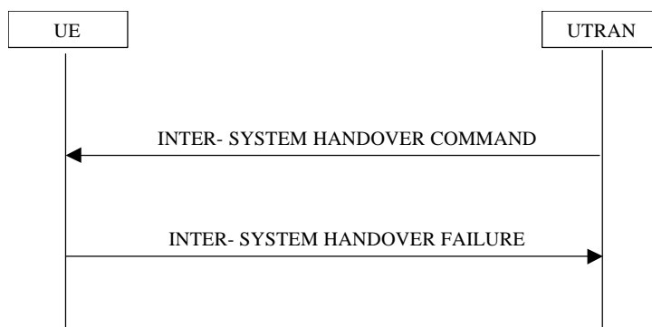
Figure 4643. Inter system handover from UTRAN, failure case
