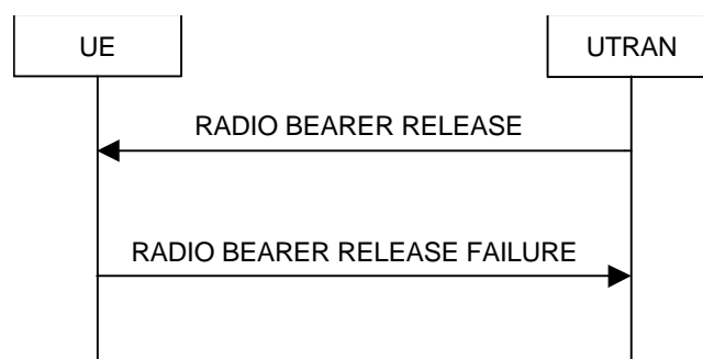
Figure 2522. Radio Bearer Release, UE reverts to old configuration
