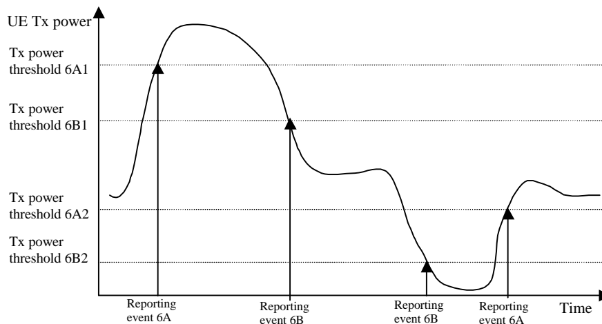
Figure 77406 Event-triggered measurement reports when the UE Tx power becomes larger or less than absolute thresholds.
