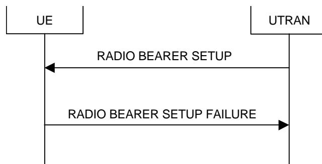
Figure 2148. Radio Bearer Establishment, UE reverts to old configuration
