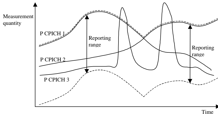
Figure 73403 Primary CPICH 3 is forbidden to affect the reporting range.
