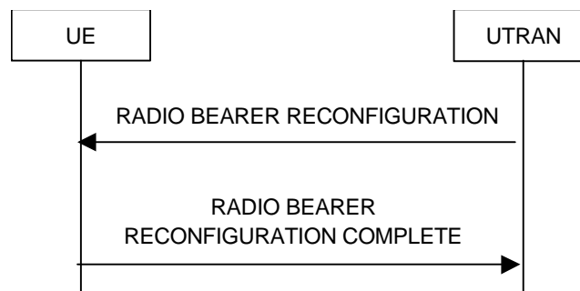
Figure 2249. Radio bearer reconfiguration, normal flow
