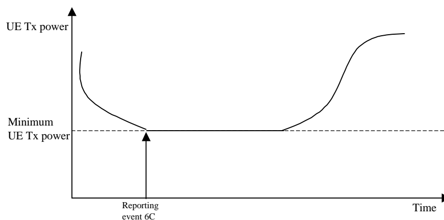
Figure 78407 Event-triggered measurement report when the UE Tx power reaches its minimum value.
