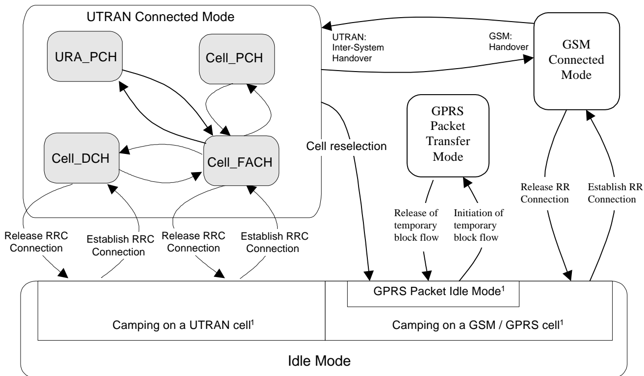
Figure 5084: RRC States and State Transitions including GSM
