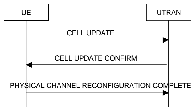
Figure 3633. Cell update procedure with physical channel reconfiguration
