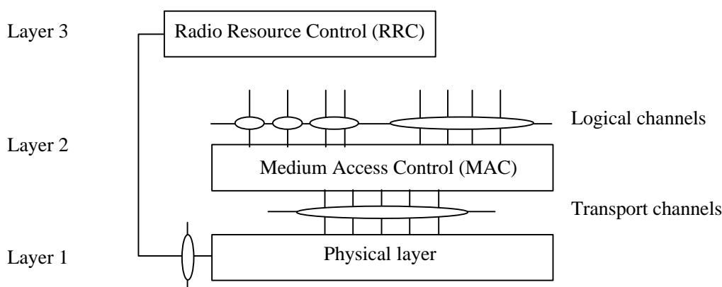
Fig. 4-1 Radio interface protocol architecture around the physical layer
