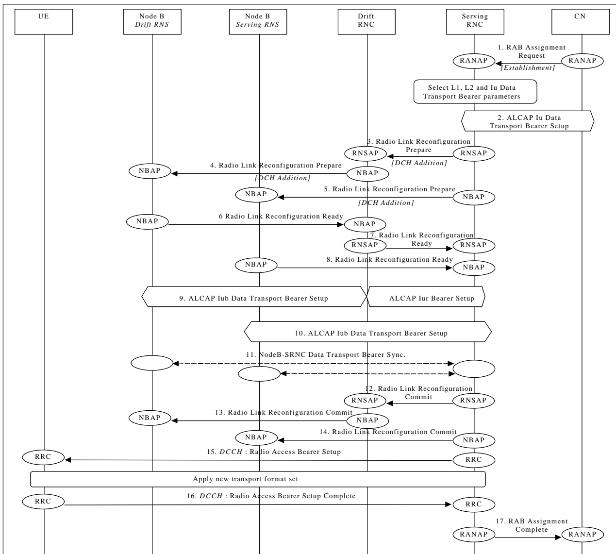
Radio Access Bearer Establishment - DCH - DCH Establishment - Synchronized
