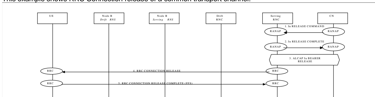
RRC Connection release of a common transport channel
