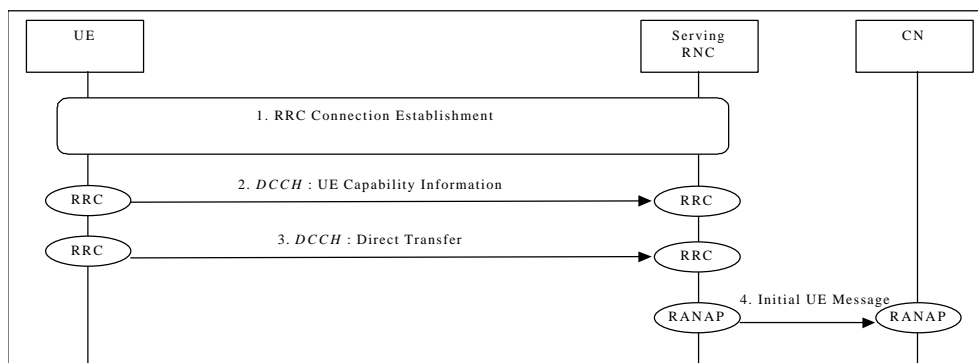
NAS Signalling Connection Establishment
