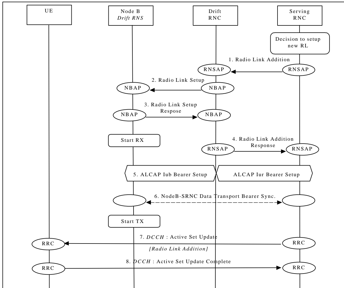
Soft Handover - Radio Link Addition (Branch Addition)
