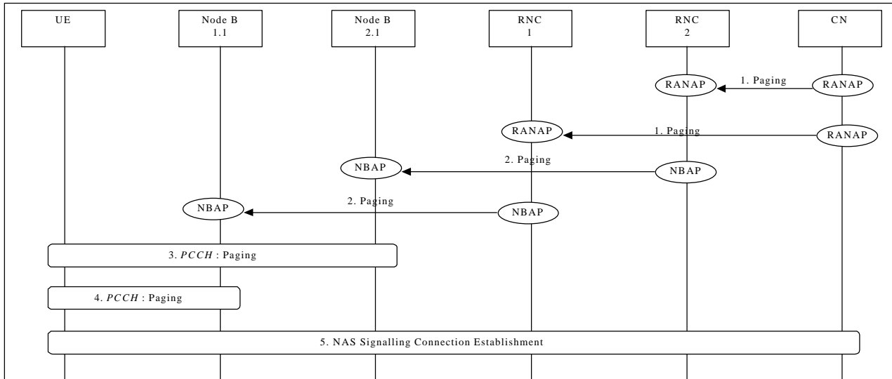
Paging for a UE in RRC Idle Mode
