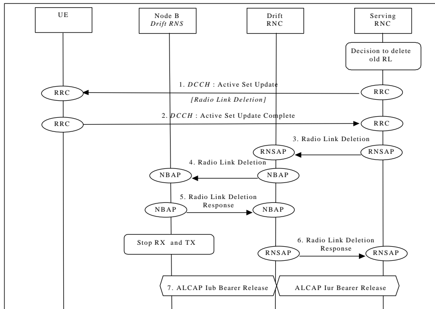
Soft Handover - Radio Link Deletion (Branch Deletion)
