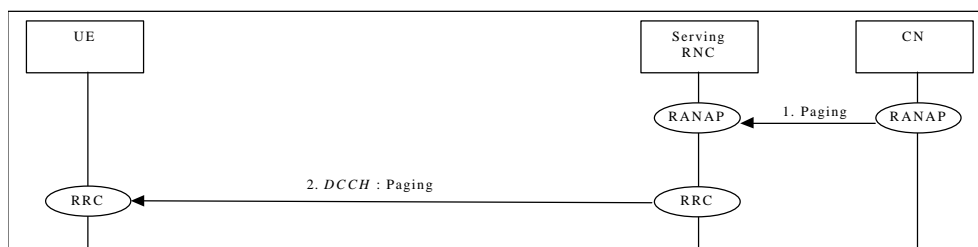
Paging for a UE in RRC Connected Mode when the UTRAN coordinates the paging request with the existing RRC connection using DCCH
