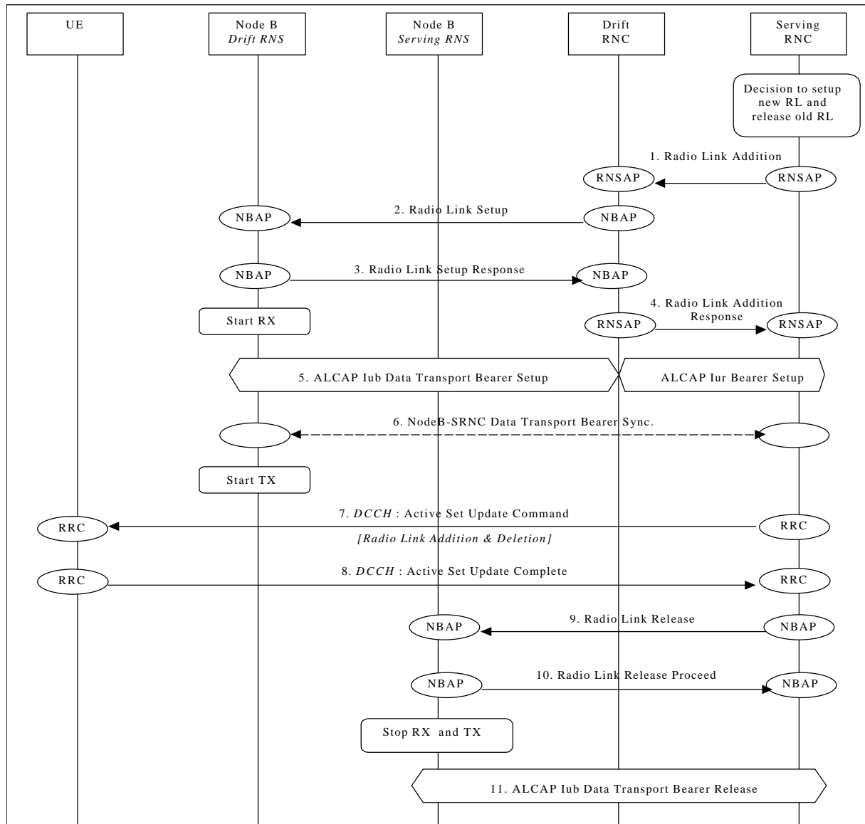
Soft Handover - Radio link Addition & Deletion (Branch Addition & Deletion - simultaneously)
