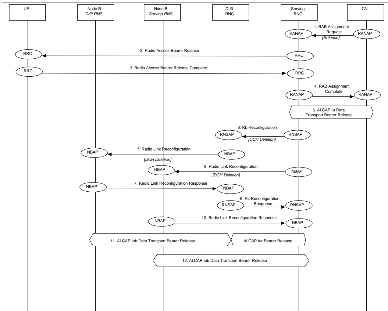
Radio Access Bearer Release - DCH - DCH Release - Unsynchronised
