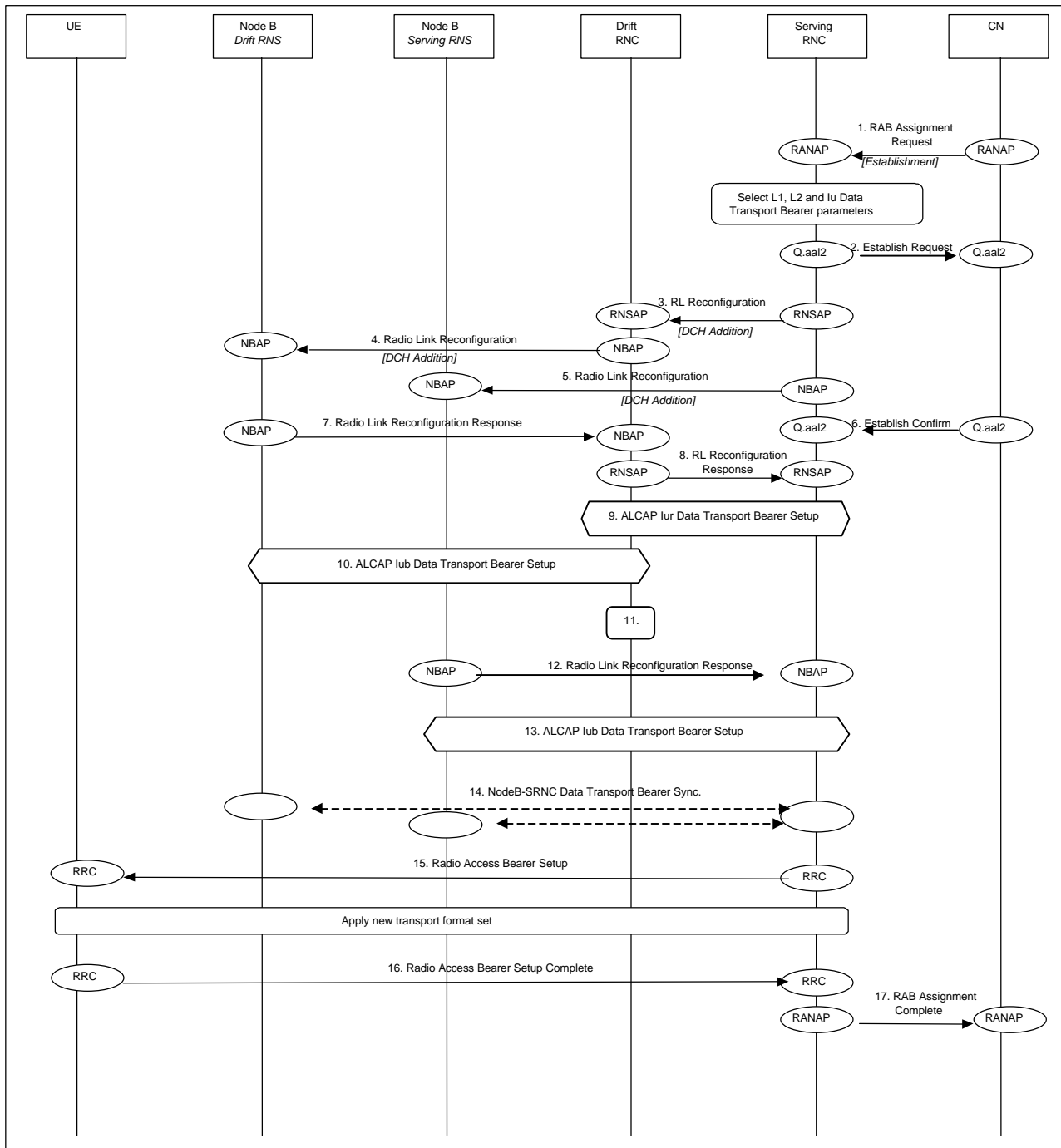
Radio Access Bearer Establishment - DCH - DCH Establishment – Unsynchronised
