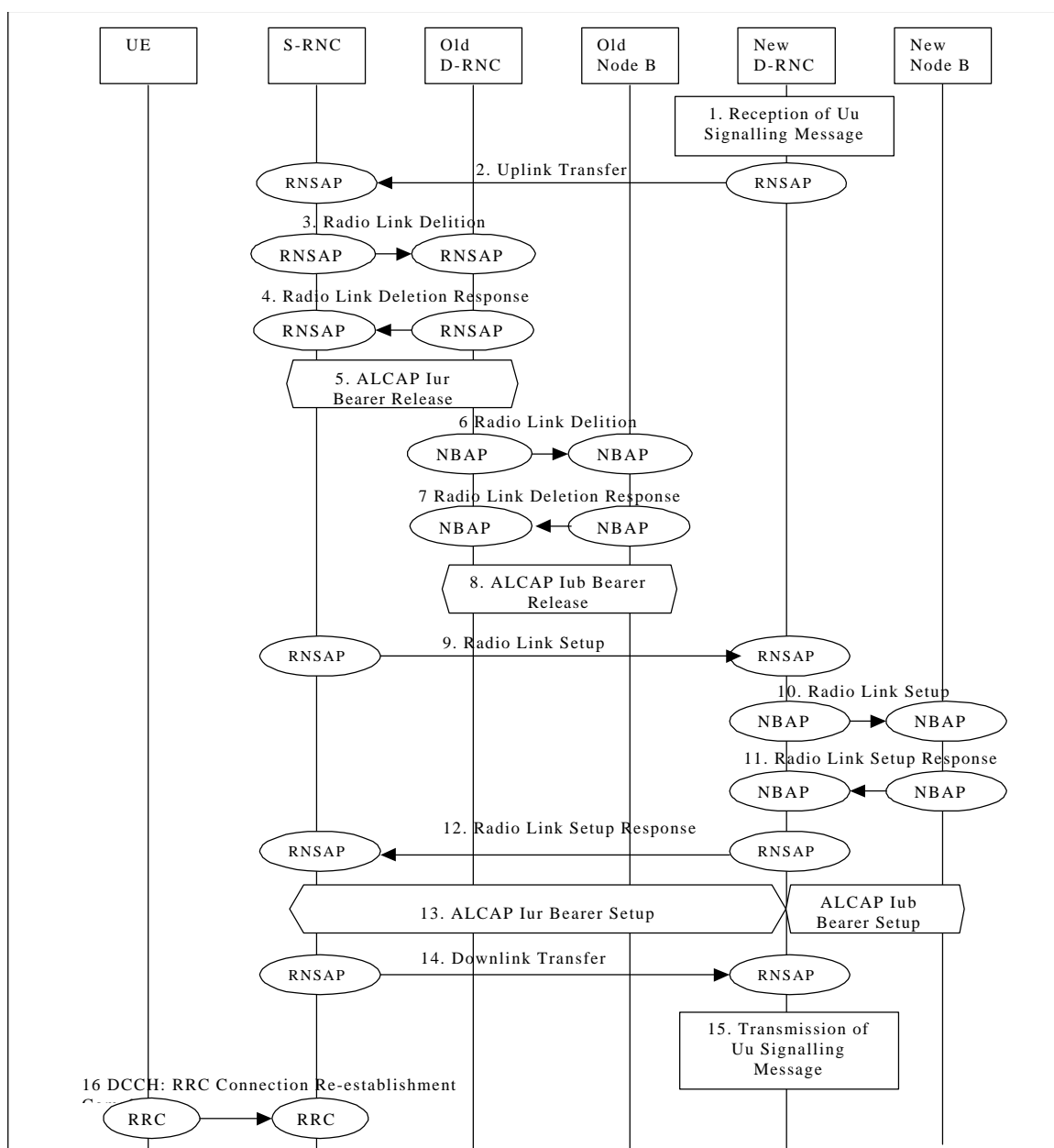
RRC connection Re-establishment (Anchor approach) – DCH Re-establishment
