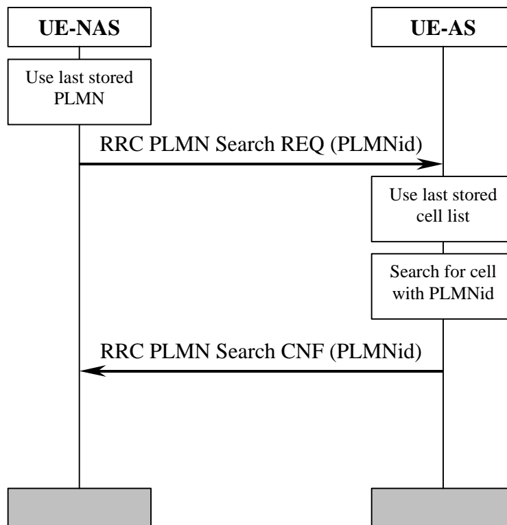
Figure 9. PLMN Selection, automatic mode, normal case.
