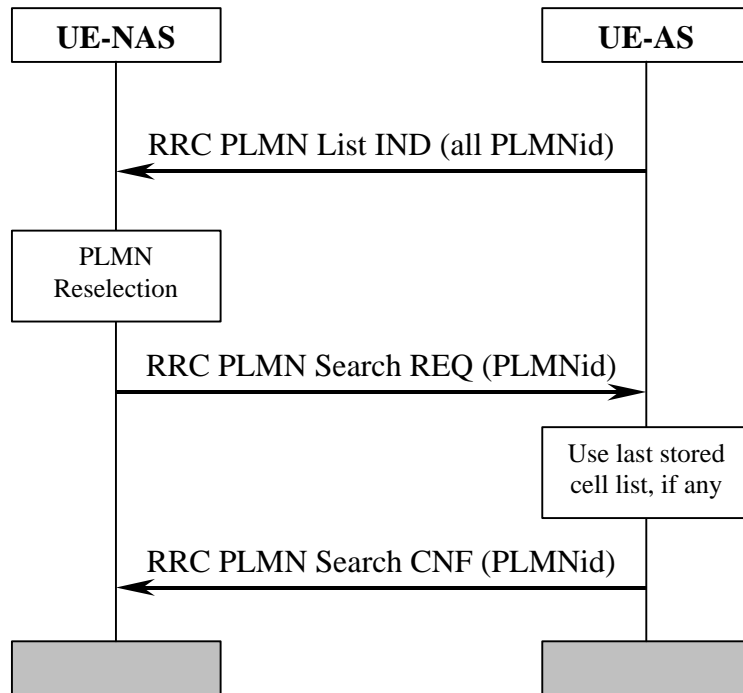
Figure 10. PLMN Reselection, automatic mode.
