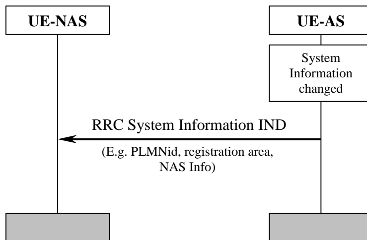
Figure 7. System Information Update to NAS.
