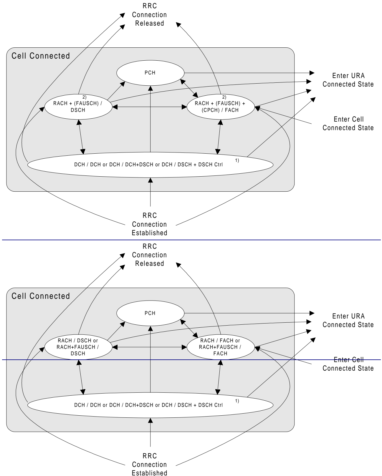
Figure 4: Substates within Cell Connected State
