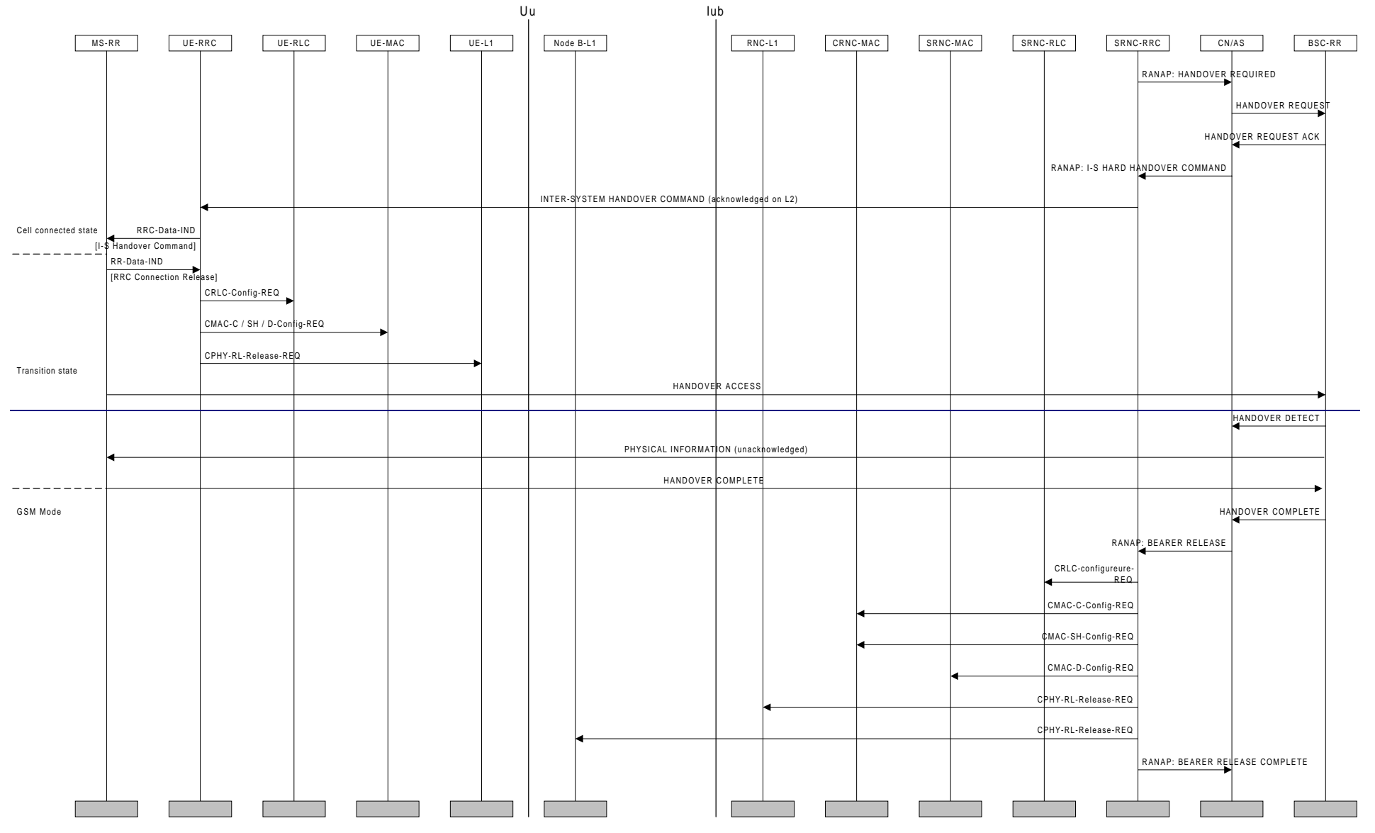
Figure 37: UTS to GSM inter-system handover
