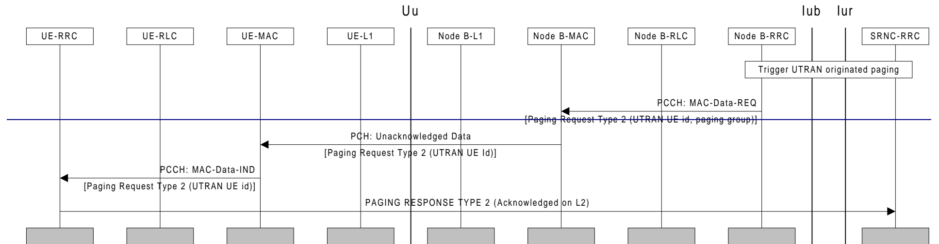
Figure 39. Example sequence for UTRAN initiated paging request with paging response
