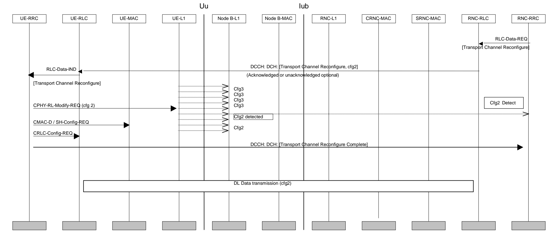
Figure 19: Asymmetric DCH Reconfiguration
