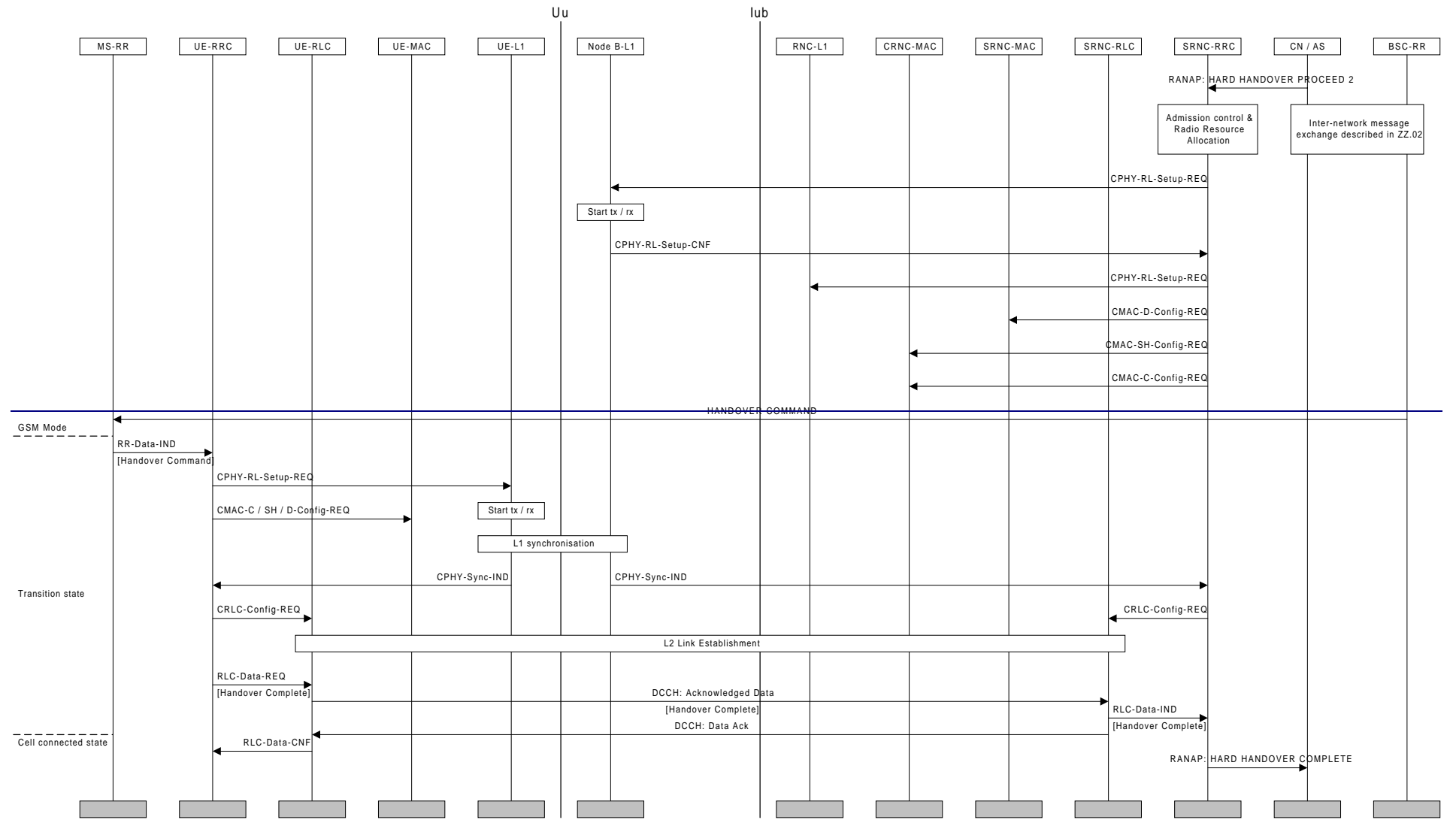
Figure 36: GSM to UMTS inter-system handover
