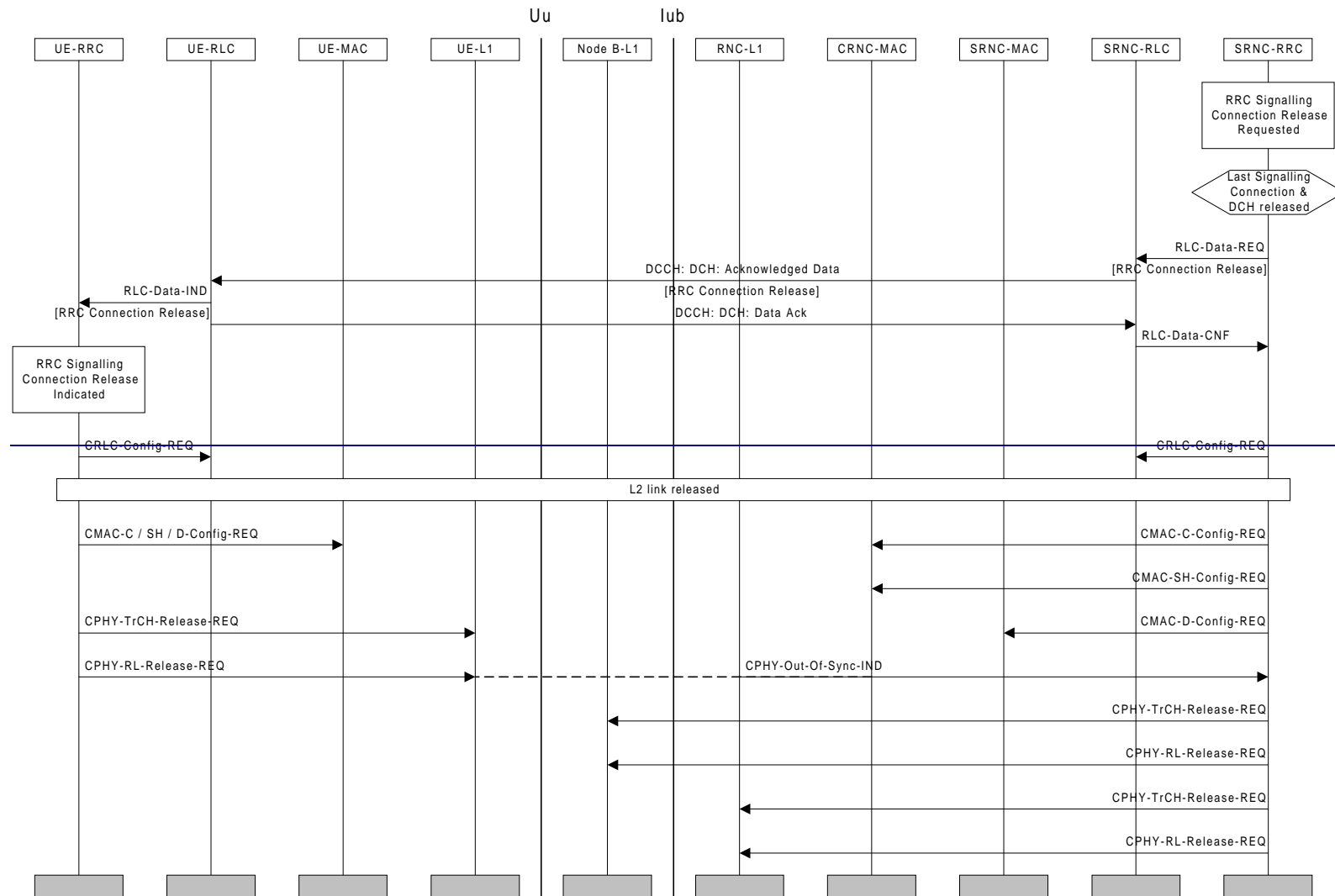
Figure 9. RRC Connection Release from Dedicated Physical Channel
