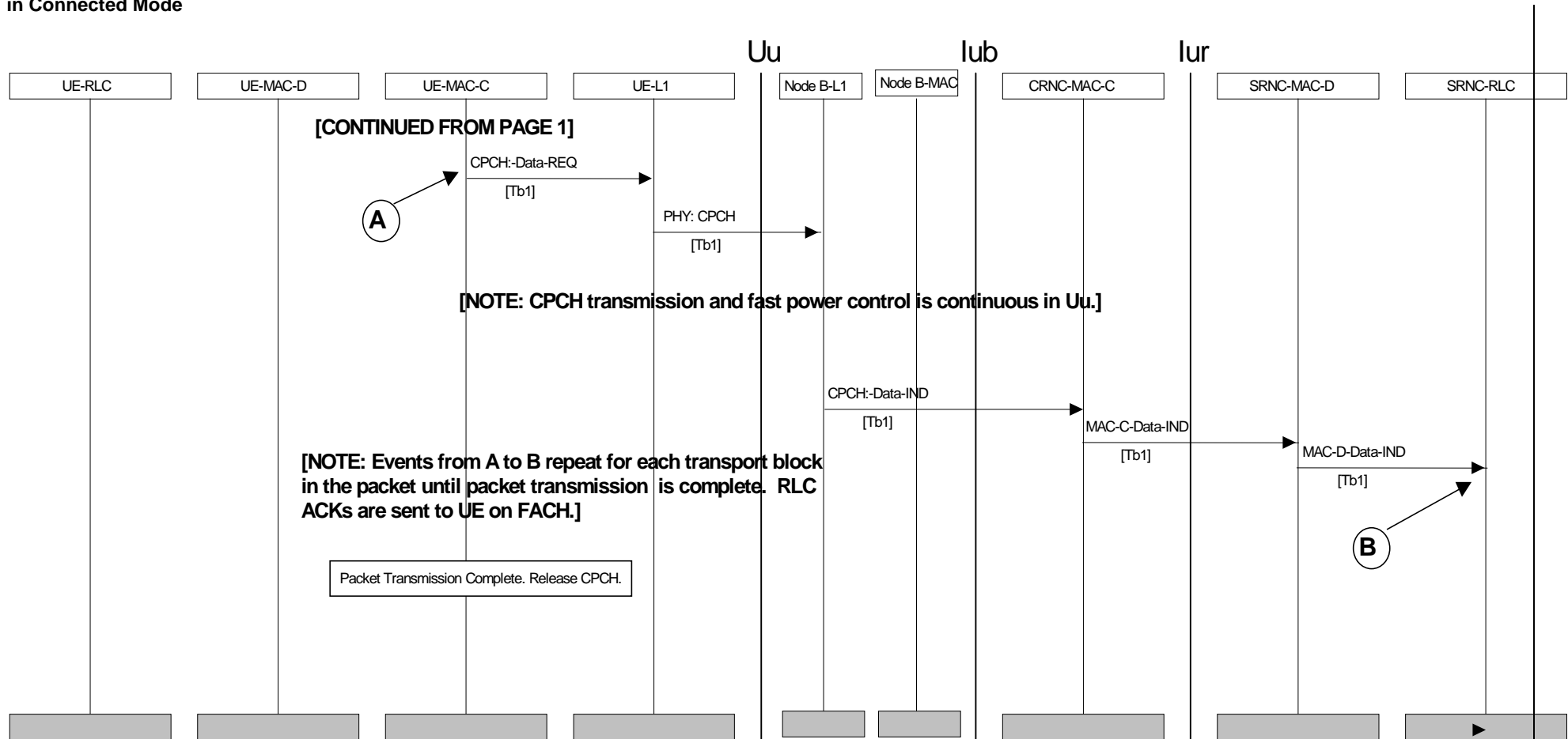
Figure 27: Example of acknowledged-mode data transmission on RACH+CPCH/FACH (page 2 of 2)
