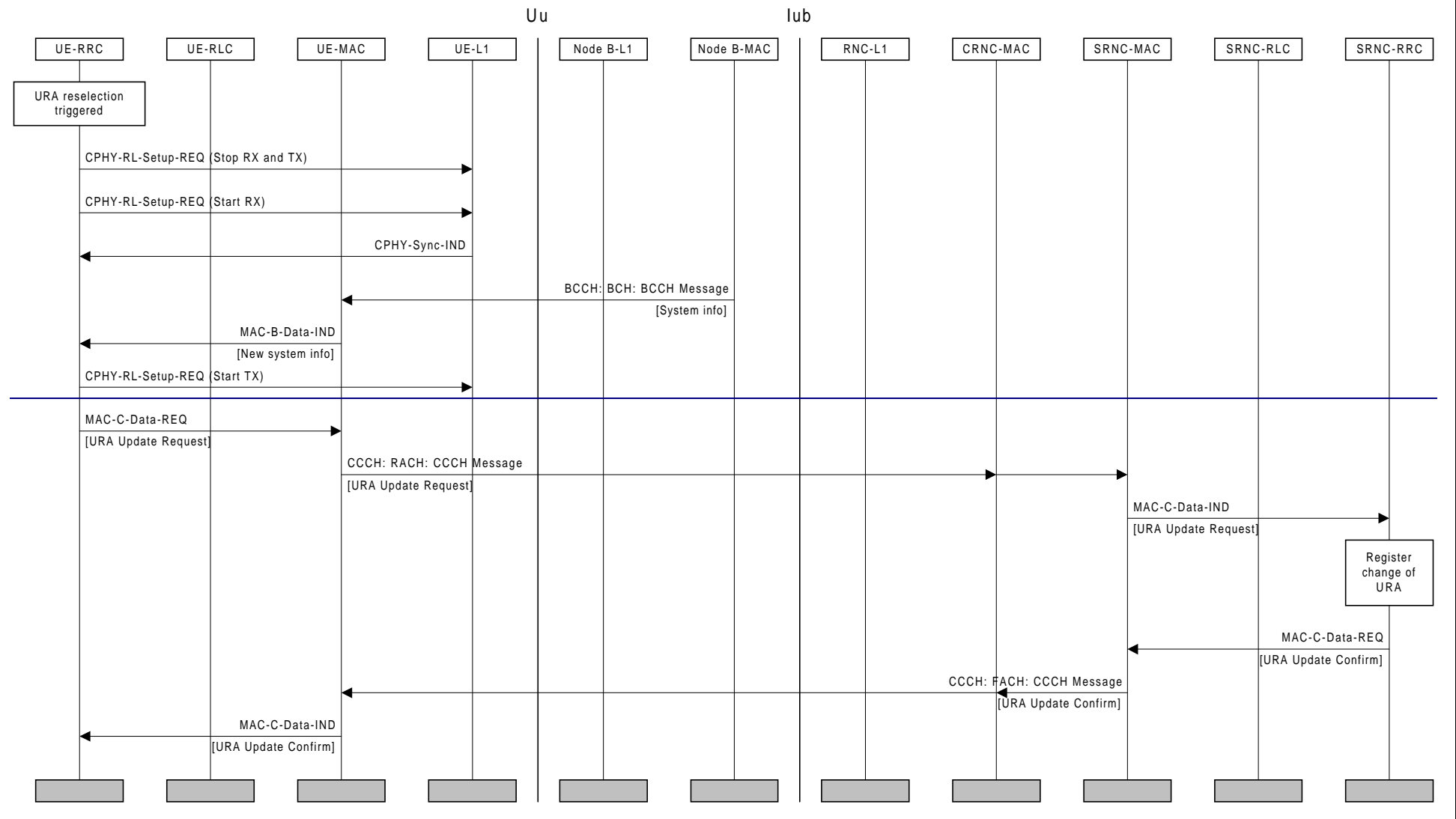
Figure 30: URA update procedure
