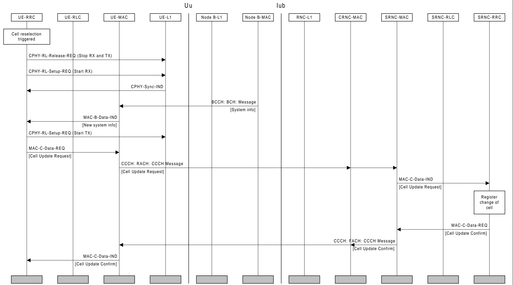
Figure 29: Cell update procedure
