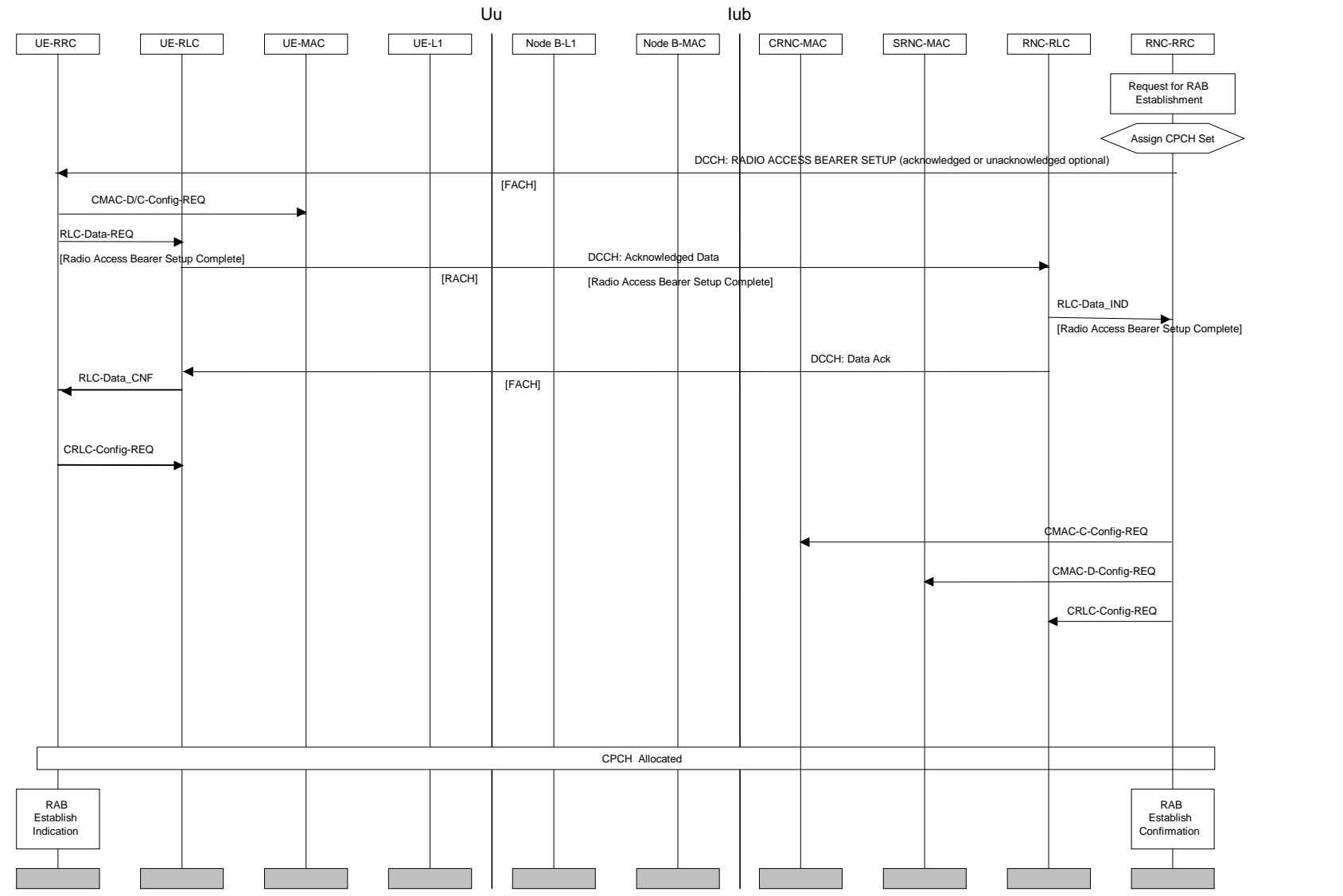
Figure 15: Radio Access Bearer Establishment with CPCH Channel Allocation
