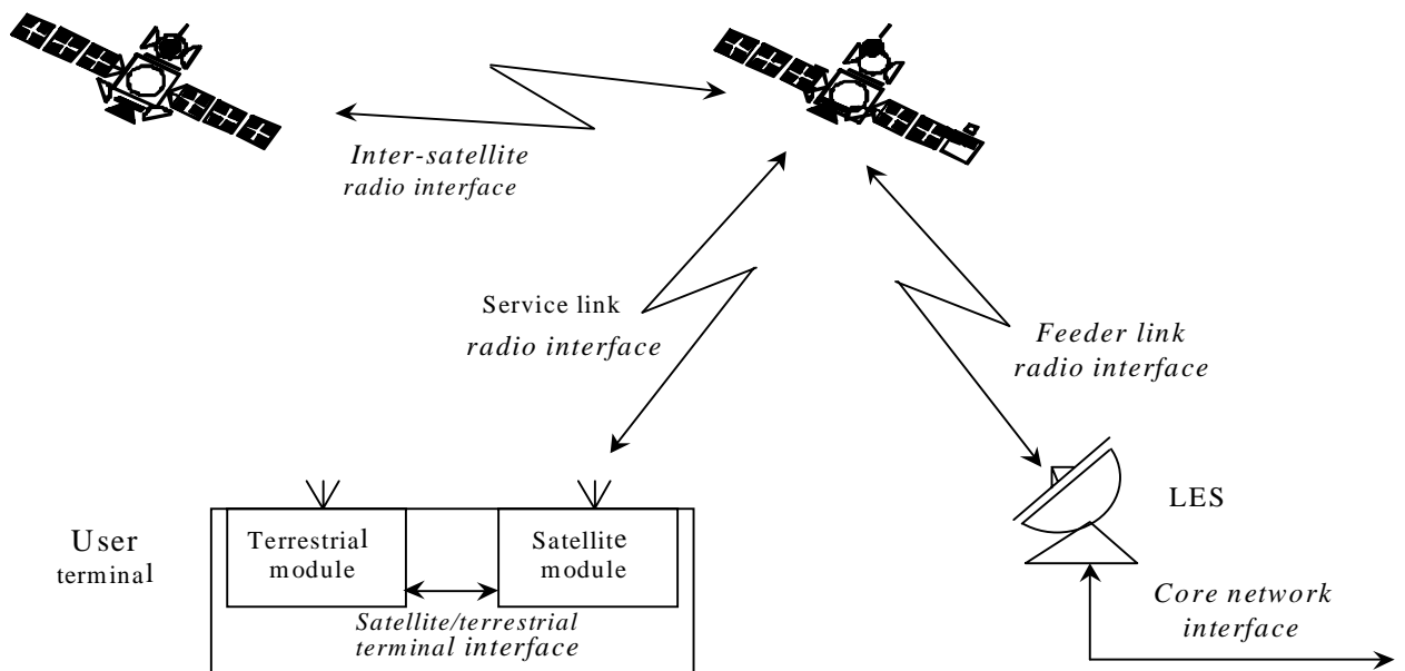
FIGURE 4.1 Interfaces in the satellite component of IMT-2000 N.B. This figure is based on Figure 1 of Recommendation ITU-R M.818
