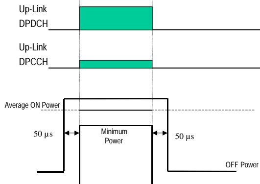
Figure 1: Transmit ON/OFF template
