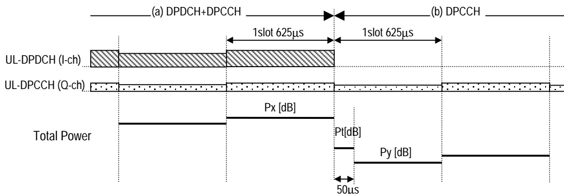
Figure xx1; Uplink Transmit DTX (DPDCH is turned OFF)
