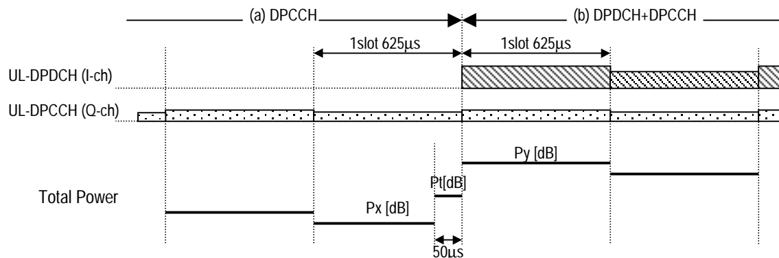
Figure xx2; Uplink Transmit DTX (DPDCH is turned ON)
