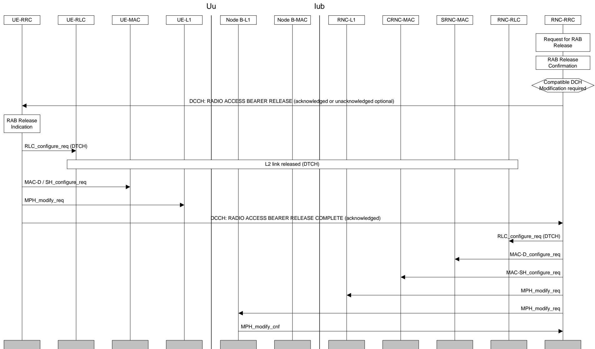
Figure Error! Unknown switch argument.: Radio Access Bearer Release with Unsynchronised Dedicated Physical Channel Modification
