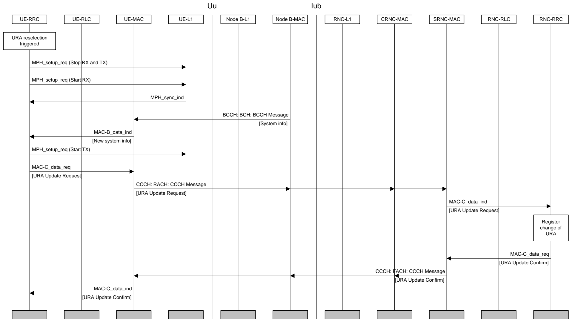
Figure Error! Unknown switch argument.: URA update procedure
