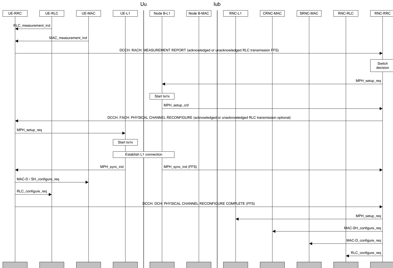
Figure Error! Unknown switch argument.: UE-Originated DCH Activation
