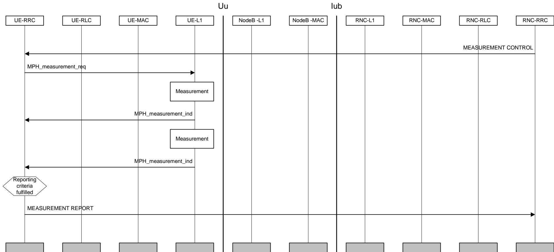
Figure Error! Unknown switch argument.: Handover measurement reporting
