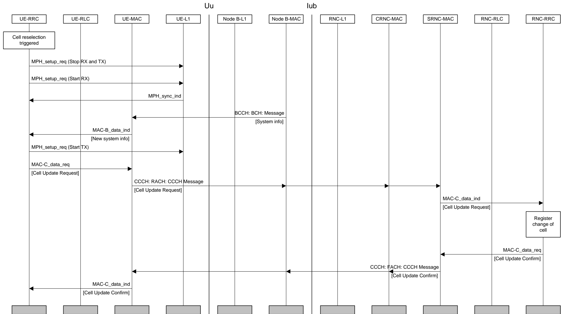
Figure Error! Unknown switch argument.: Cell update procedure
