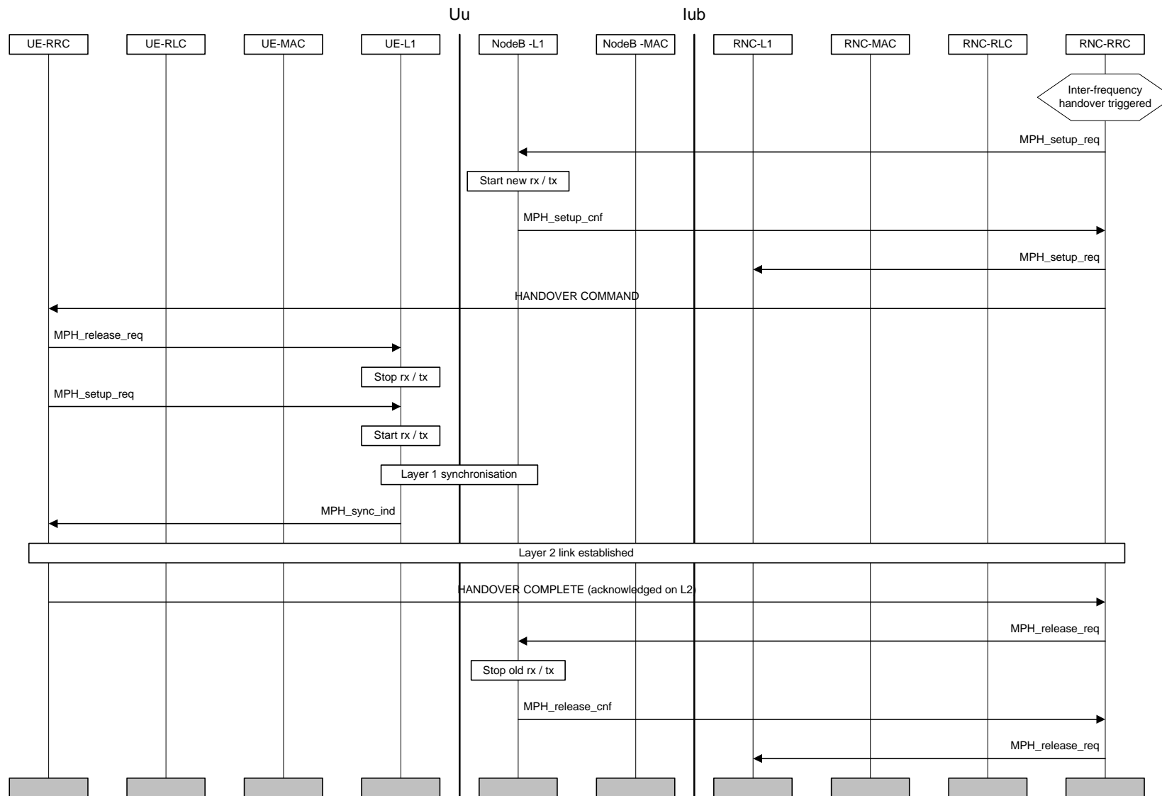
Figure Error! Unknown switch argument.: Hard handover
