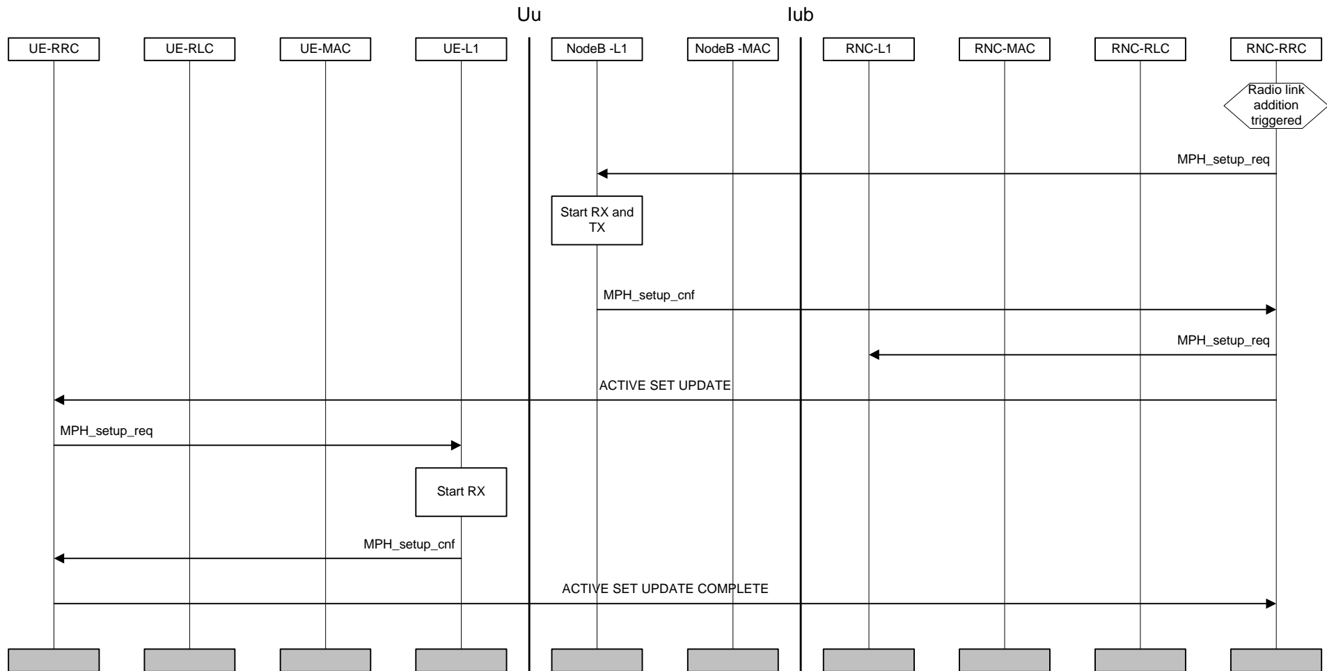
Figure Error! Unknown switch argument.: Radio Link Addition
