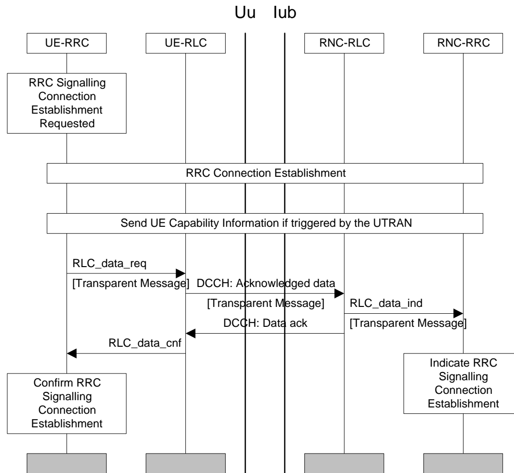
Figure Error! Unknown switch argument.. UE initiated Signalling Connection Establishment
