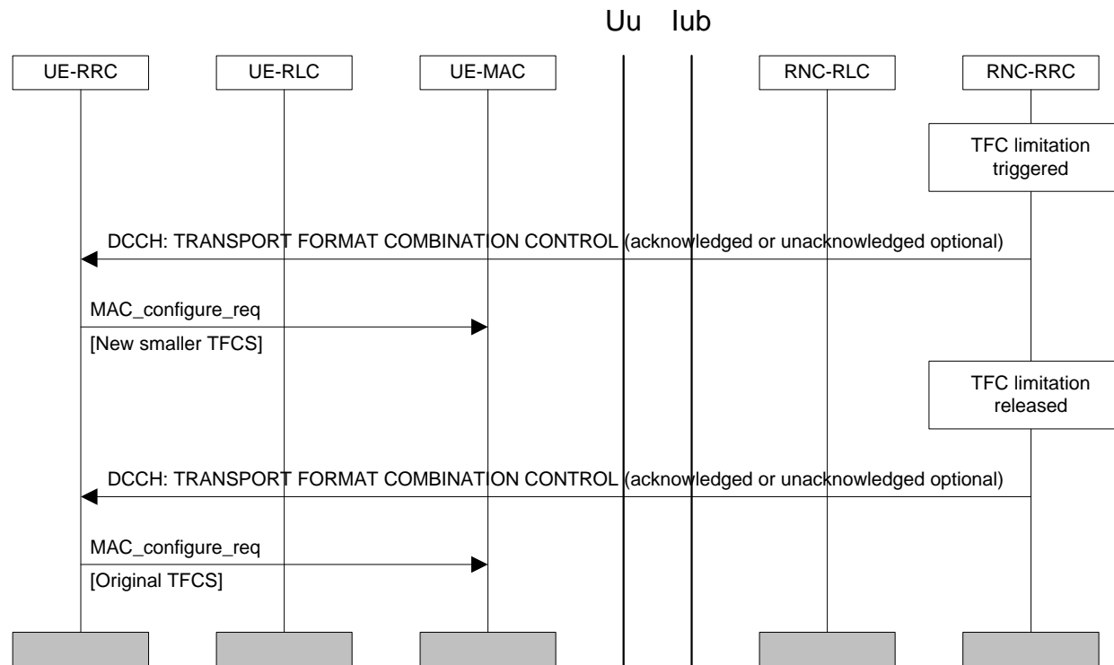
Figure Error! Unknown switch argument.: Transport Format Combination Limitation
