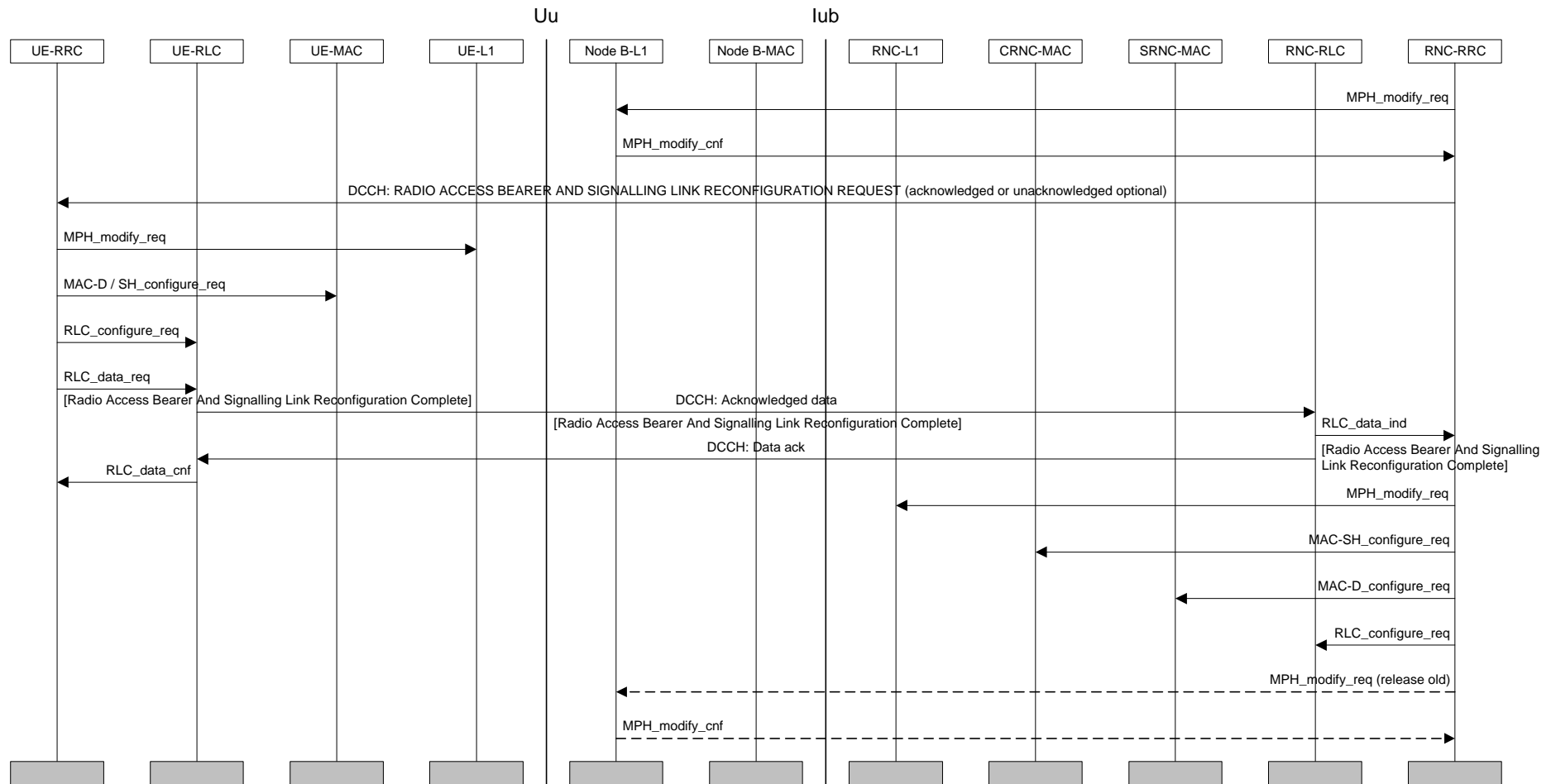
Figure Error! Unknown switch argument.: Unsynchronised Radio Access Bearer Reconfiguration
