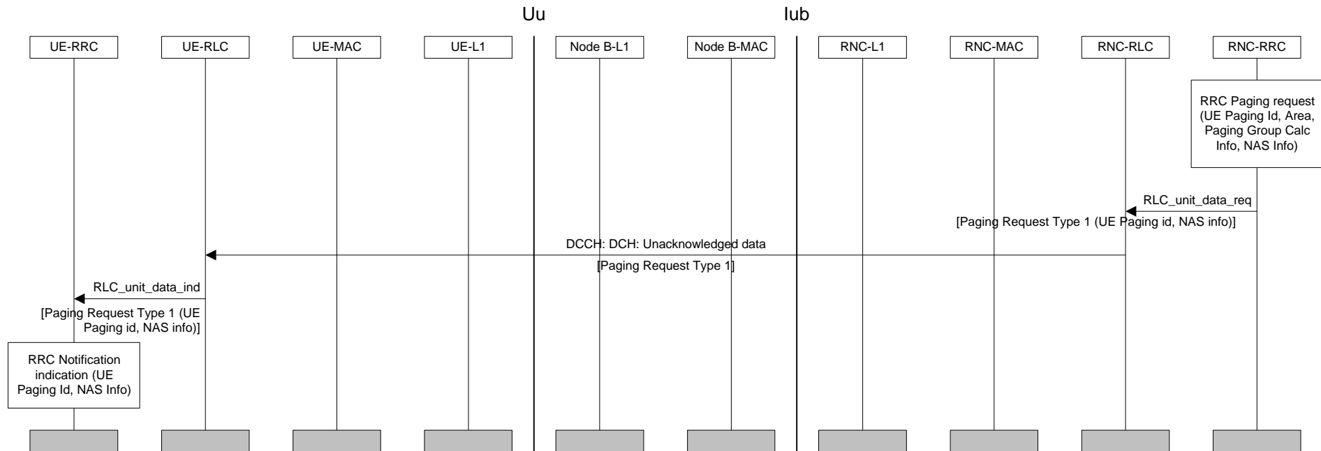
Figure Error! Unknown switch argument.. Example sequence of CN initiated paging request using DCCH
