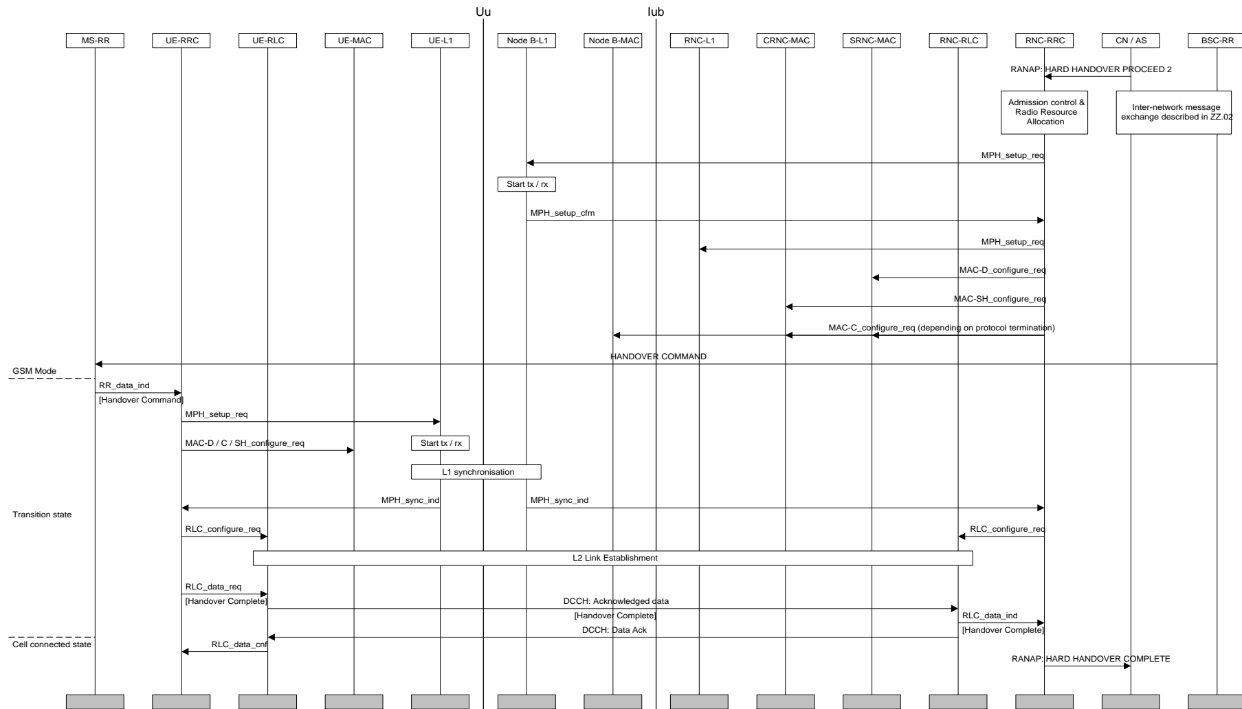
Figure Error! Unknown switch argument : GSM to UMTS inter-system handover
