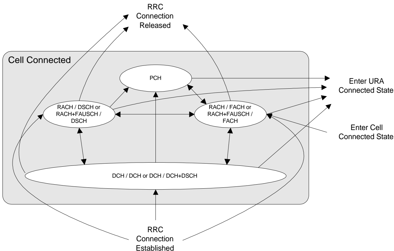
Figure Error! Unknown switch argument.: Substates within Cell Connected State
