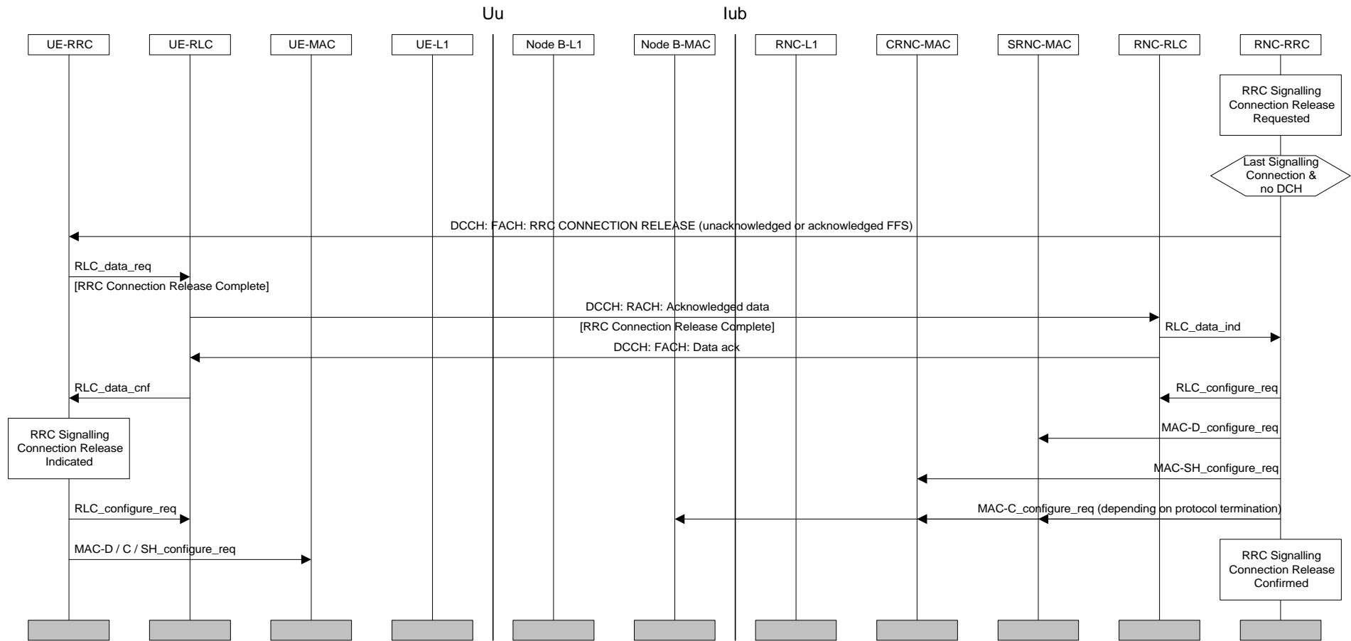
Figure Error! Unknown switch argument.: RRC Connection Release without Dedicated Physical Channel
