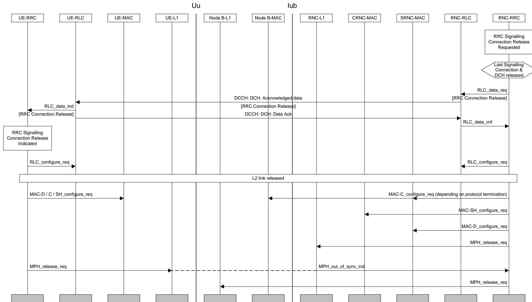
Figure Error! Unknown switch argument.. RRC Connection Release from Dedicated Physical Channel
