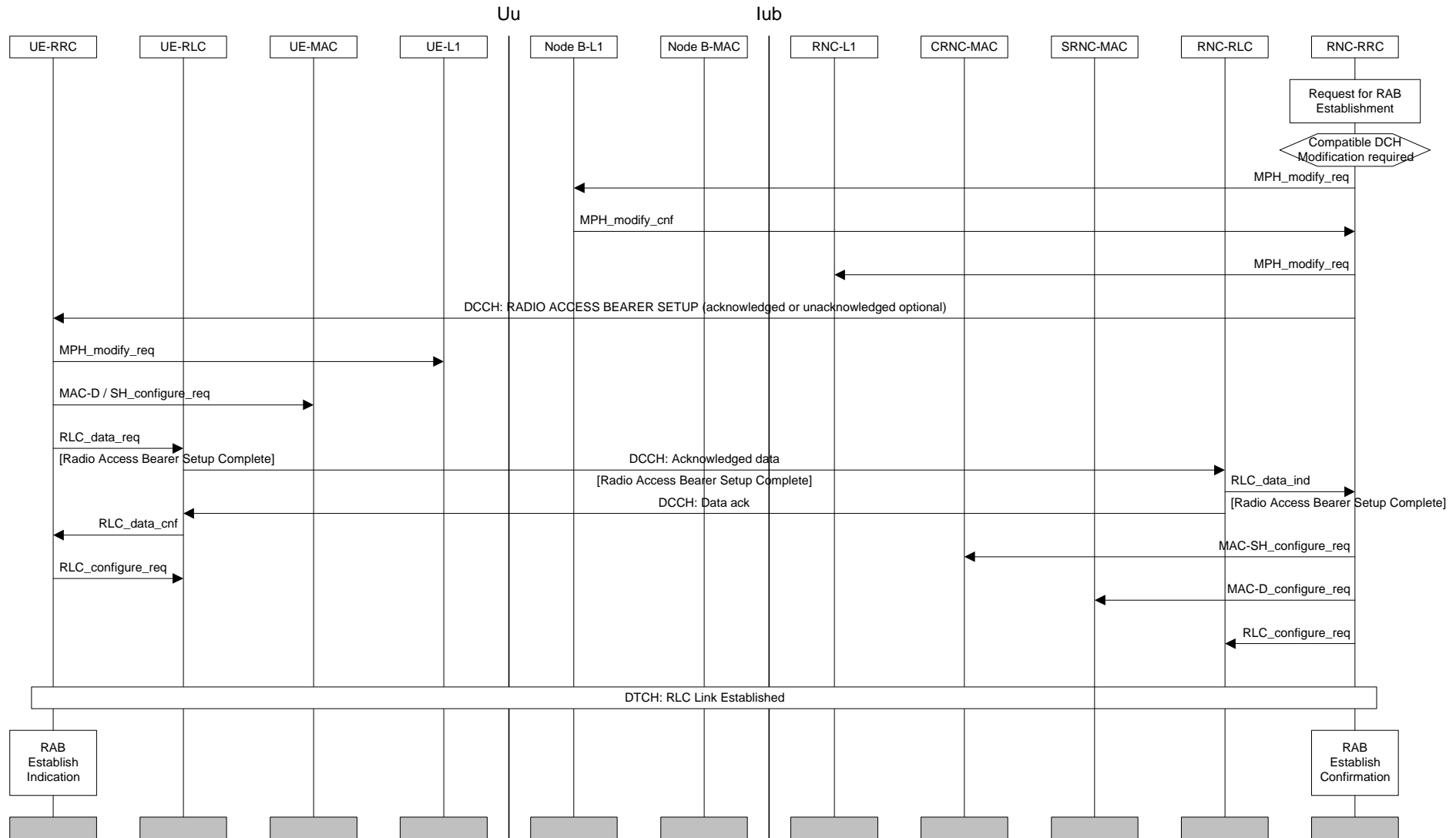
Figure Error! Unknown switch argument.: Radio Access Bearer Establishment with Unsynchronised Dedicated Physical Channel Modification
