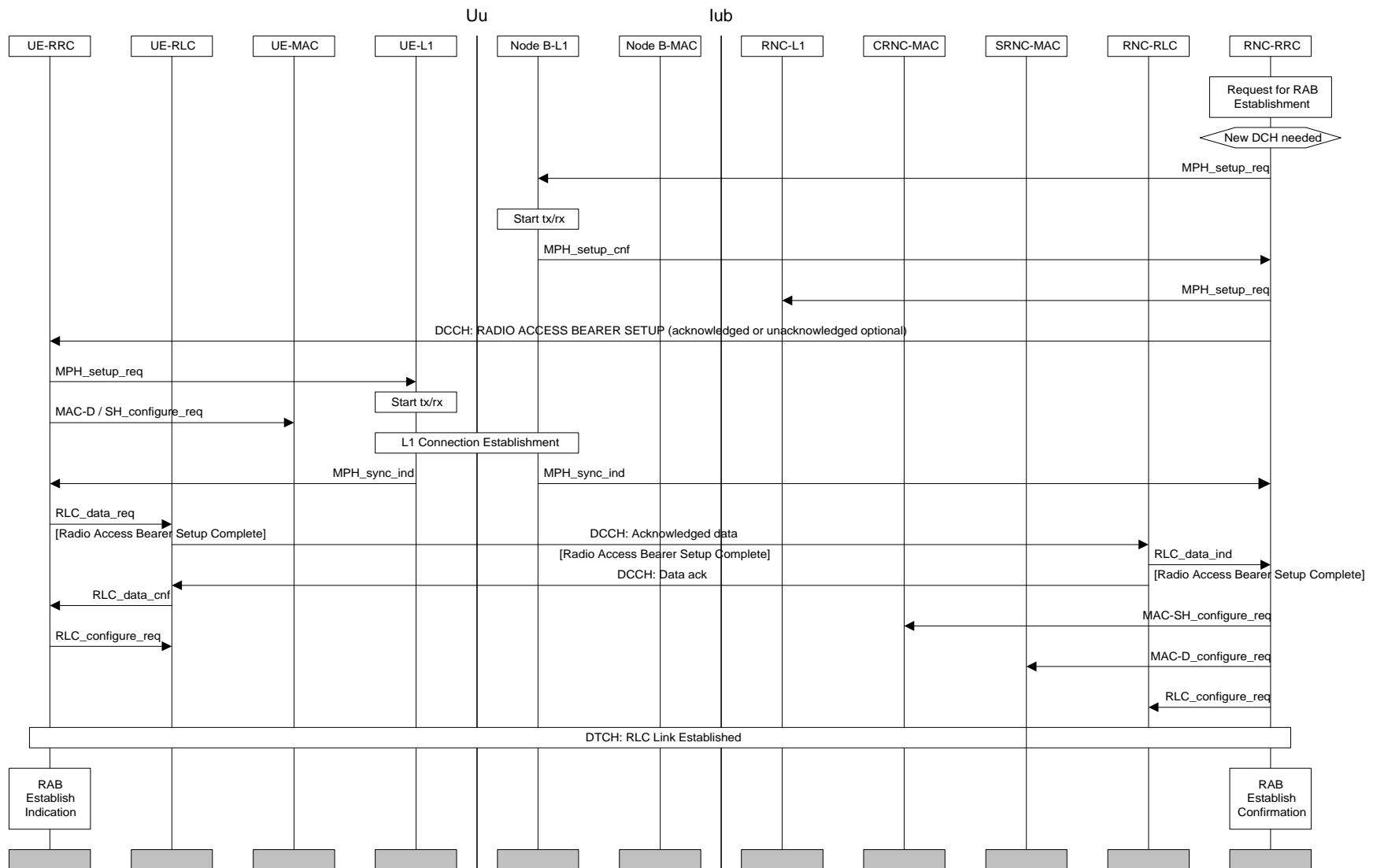
Figure Error! Unknown switch argument.: Radio Access Bearer Establishment with Dedicated Physical Channel Activation
