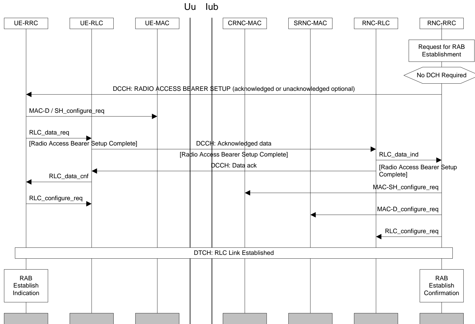
Figure Error! Unknown switch argument.: Radio Access Bearer Establishment without Dedicated Physical Channel
