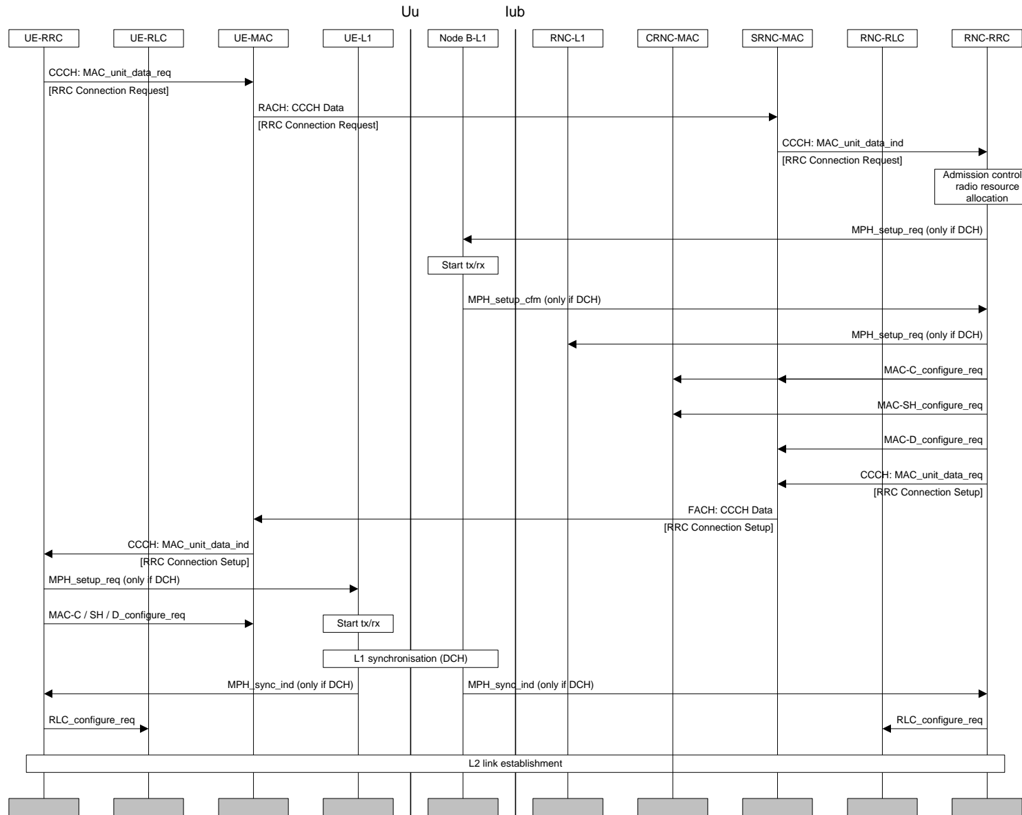
Figure Error! Unknown switch argument.. RRC connection establishment with common channel termination case A
