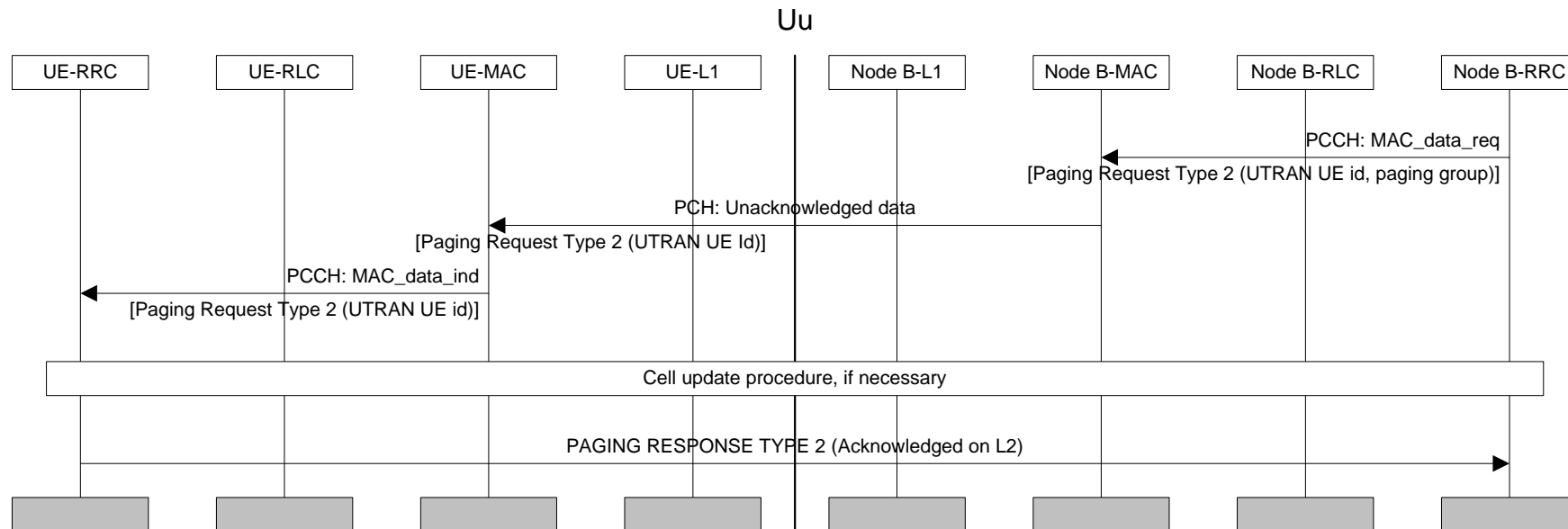
Figure Error! Unknown switch argument.. Example sequence for UTRAN initiated paging request with paging response
