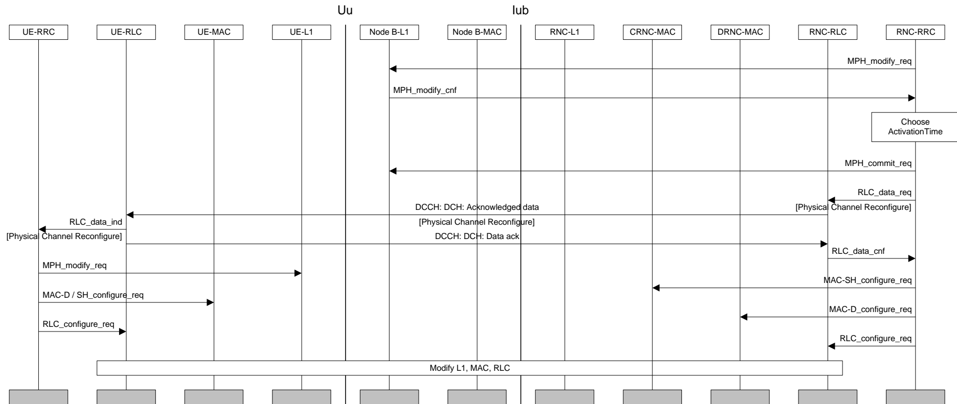
Figure Error! Unknown switch argument.: UE-terminated synchronised DCH Modify
