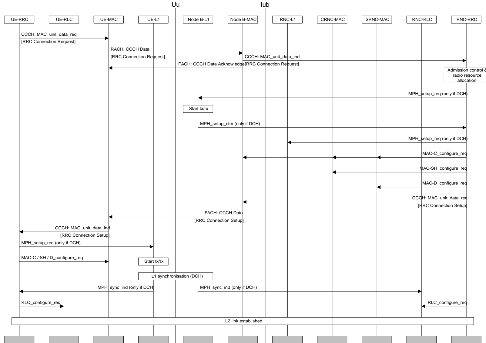
Figure Error! Unknown switch argument.: RRC connection establishment with common channel termination case C
