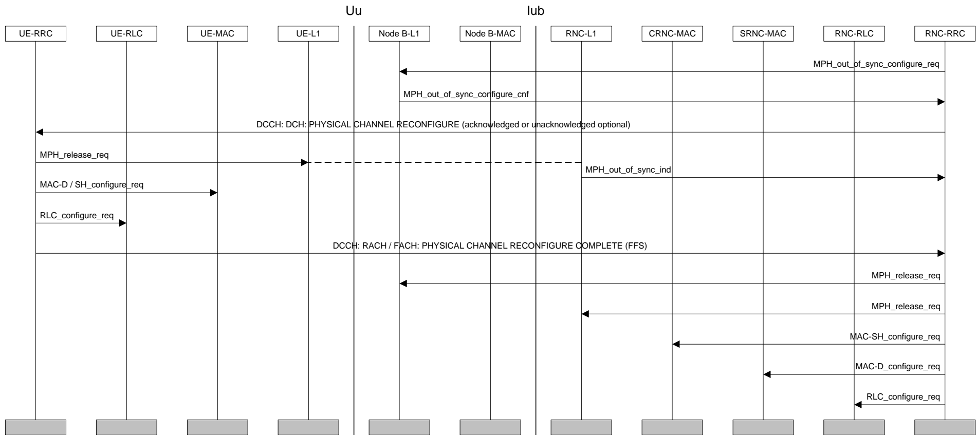
Figure Error! Unknown switch argument.: UE-terminated DCH Release
