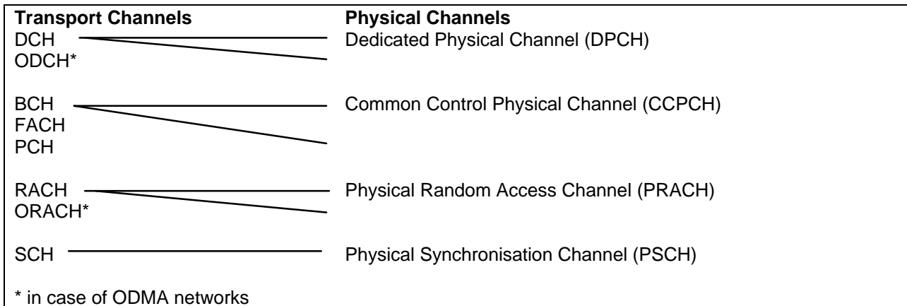
Figure 14 Transport channel to physical channel mapping
