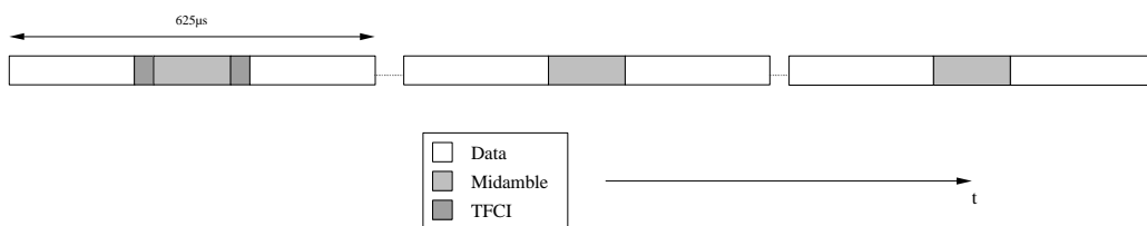
Figure 9 Example of TFCI transmission with RUs multiplexed in time domain
