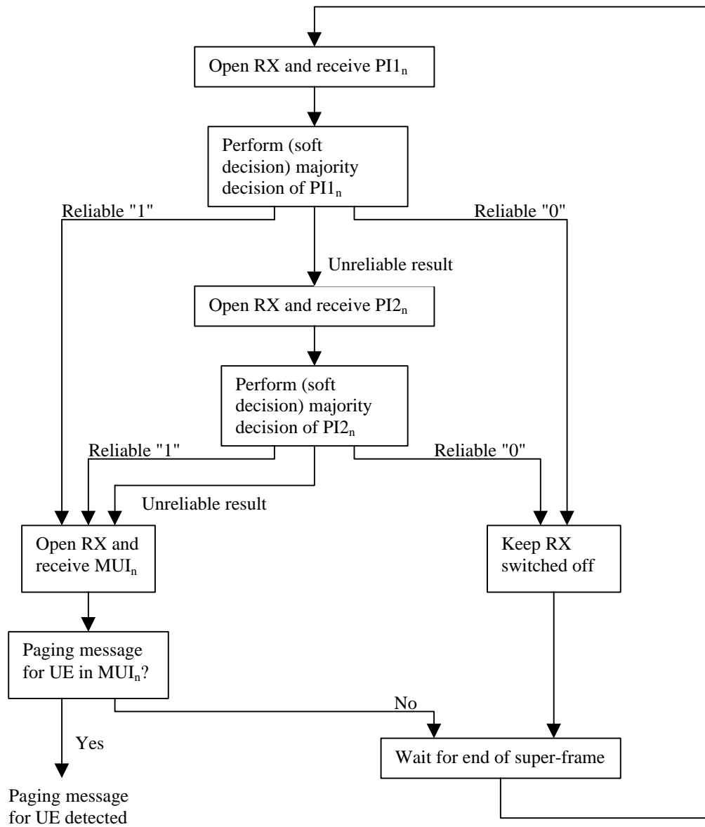
Figure 8: Detection of paging messages.
