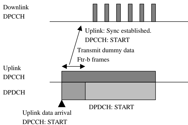
Figure 7: Transmission resumption of downlink DPDCH
