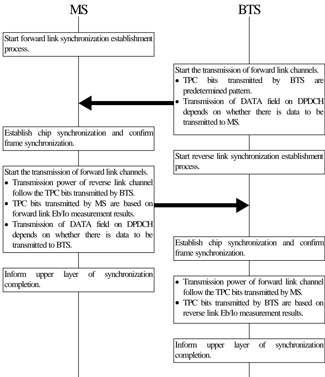
Fig.3.2.6-1 Synchronization Establishment Flow of Dedicated Channels
