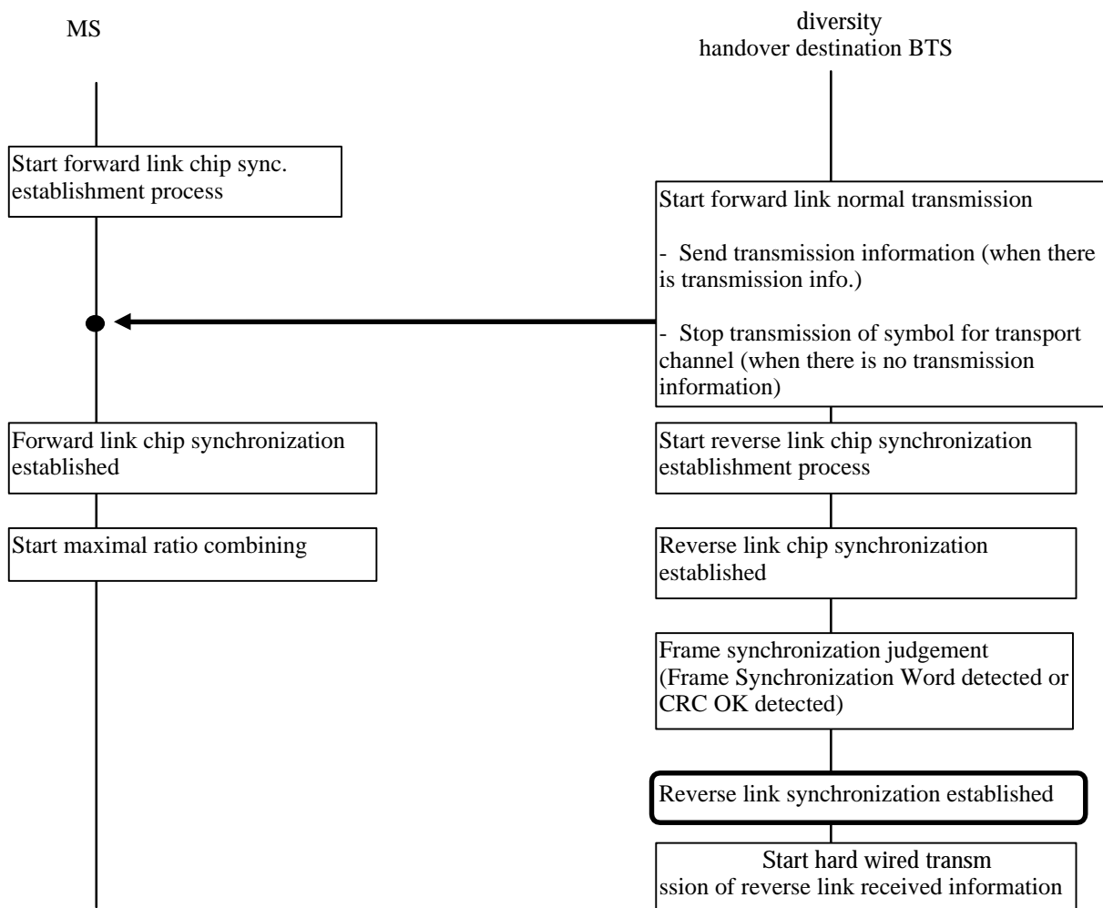
Fig. 3.2.6-4 Synchronization Establishment Flow Upon Intra/Inter-cell Diversity Handover
