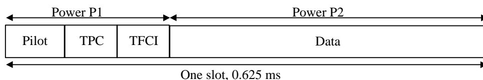
Figure 3: Power setting of the downlink Dedicated Physical Channel
