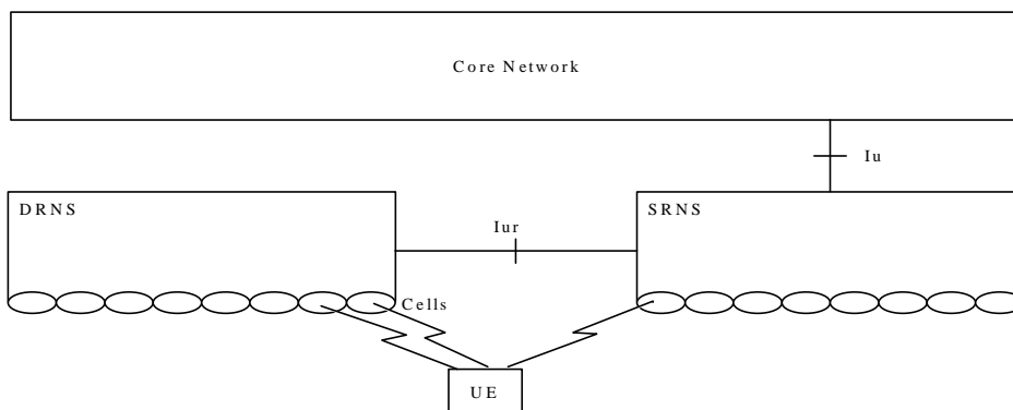
Figure 3. Serving and Drift RNS
