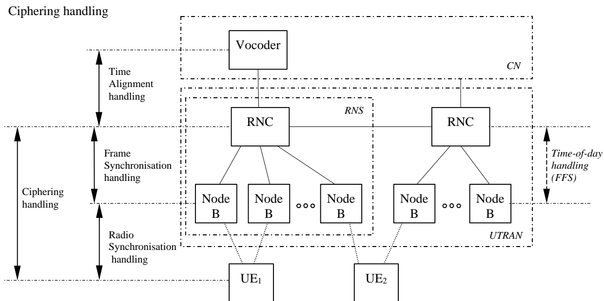
Figure 6. Synchronisation issues model.
