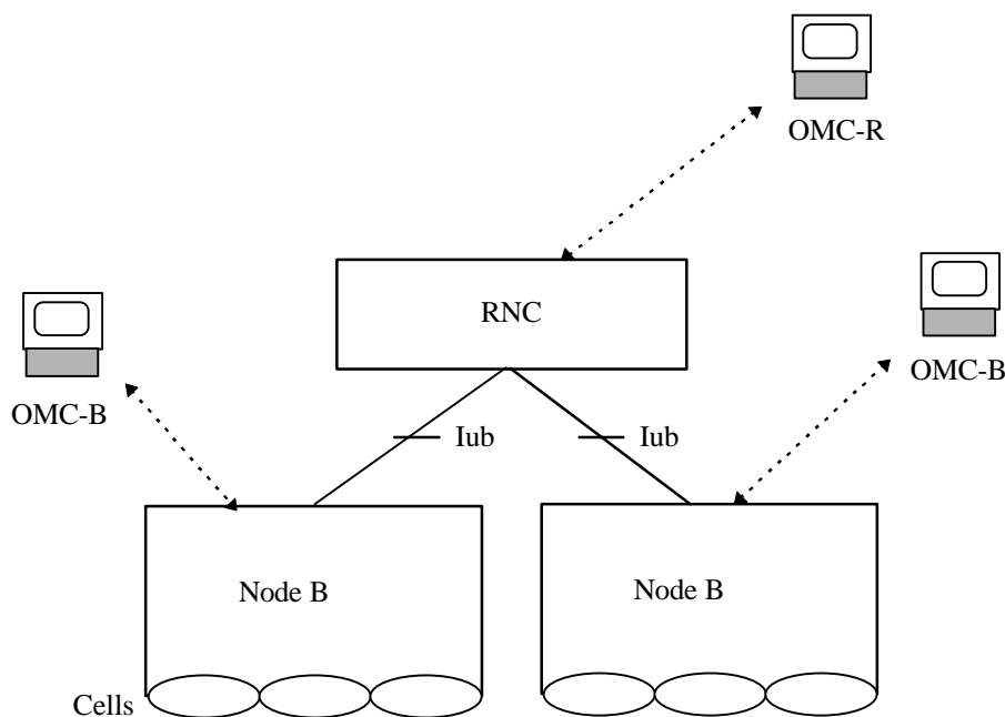
Figure 4. RNS architecture with O&M interfaces
