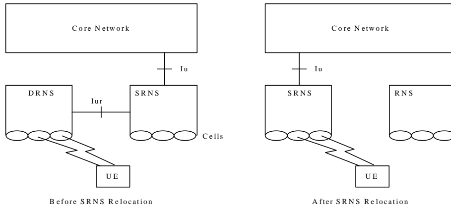
Figure 15. Serving RNS Relocation
