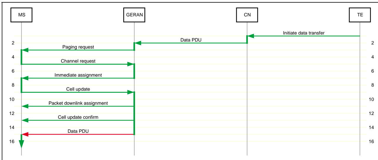
Figure 15: Incoming packet data transfer – RRC-GRA_PCH, CCCH, assign shared channel
