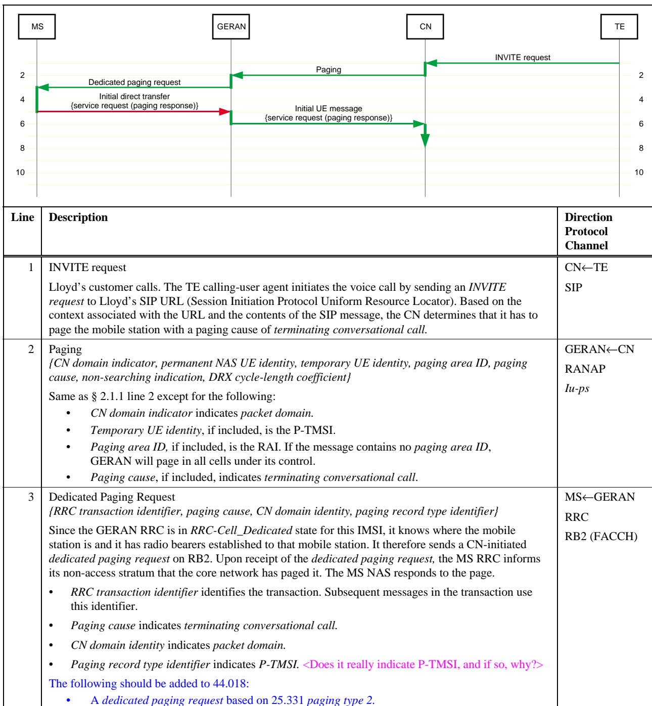
Figure 6: Incoming packet voice call – RRC-Cell_Dedicated, assign dedicated channel
