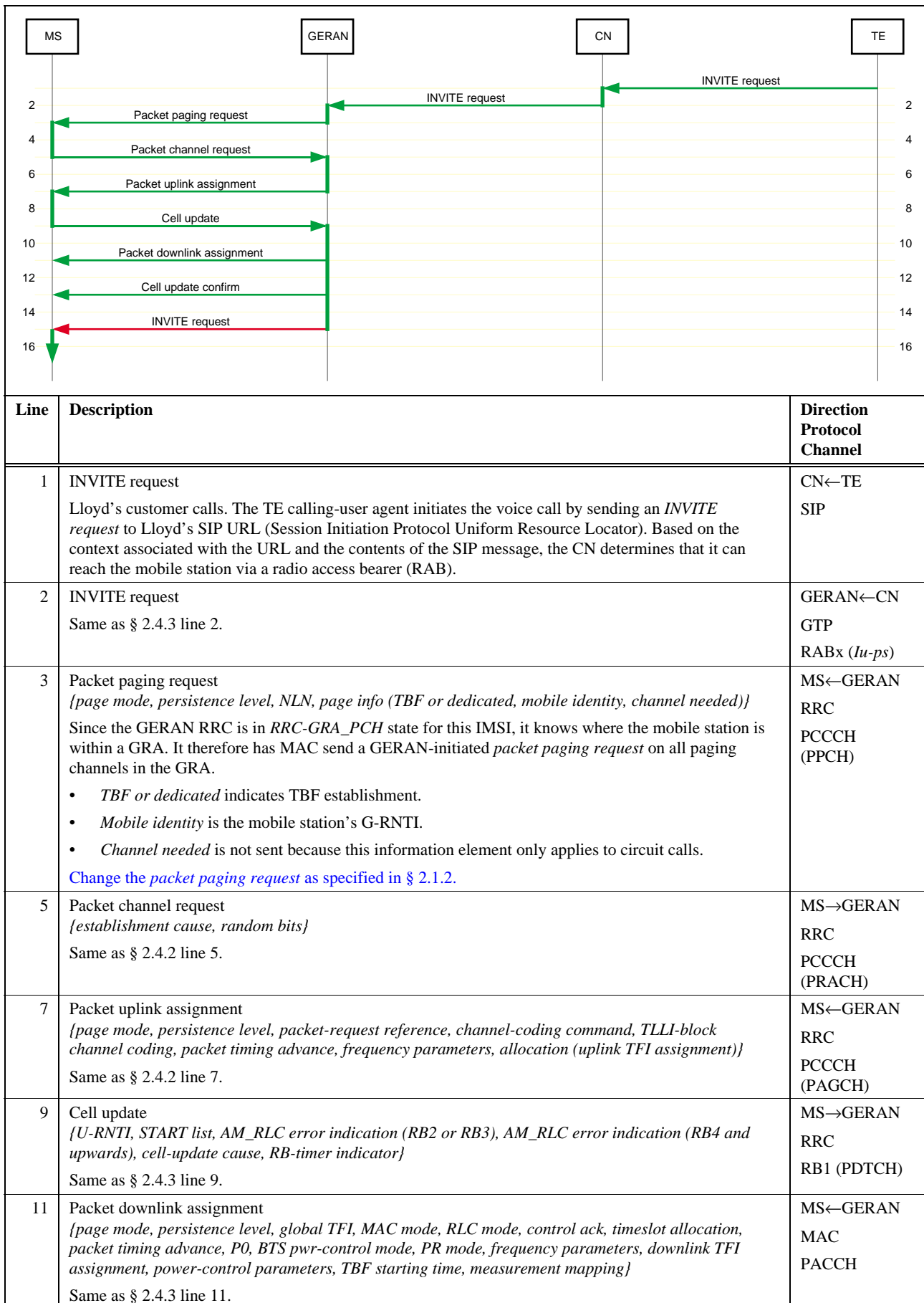
Figure 11: Incoming packet voice call – RRC-GRA_PCH, PCCCH, assign shared channel
