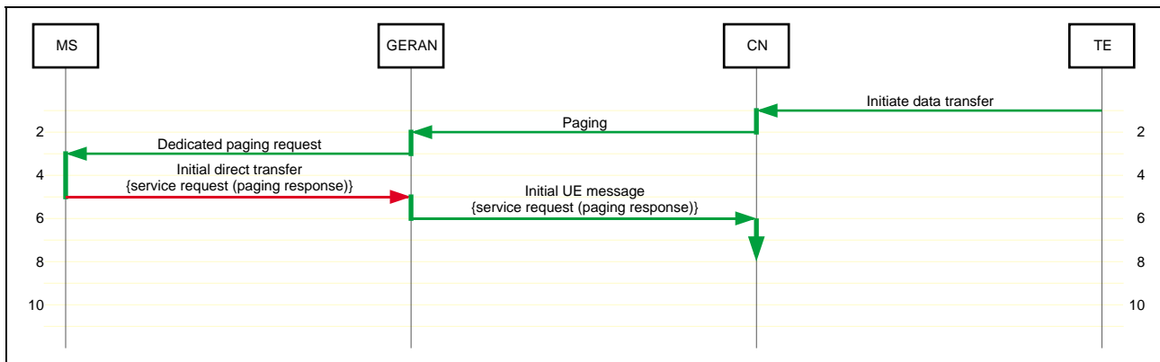
Figure 12: Incoming packet data transfer – RRC-Cell_Dedicated , assign dedicated channel
