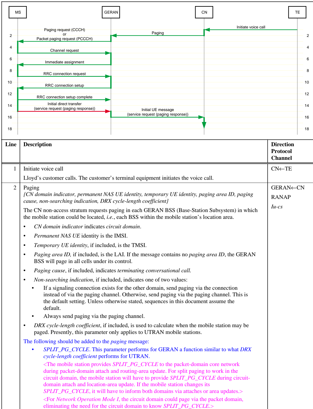
Figure 1: Incoming circuit voice call – RRC-Idle, assign dedicated channel
