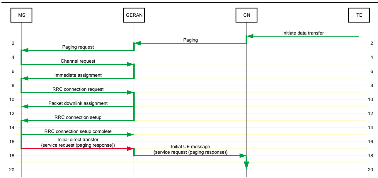
Figure 13: Incoming packet data transfer – RRC-Idle, CCCH, assign shared channel
