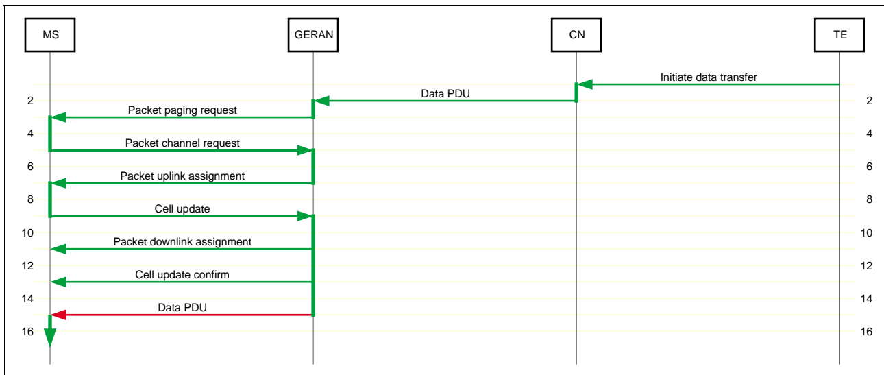
Figure 16: Incoming packet data transfer – RRC-GRA_PCH, PCCCH, assign shared channel
