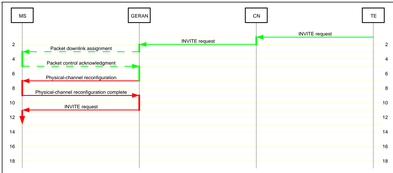
Figure 5: Incoming packet voice call – RRC-Shared, assign dedicated channel
