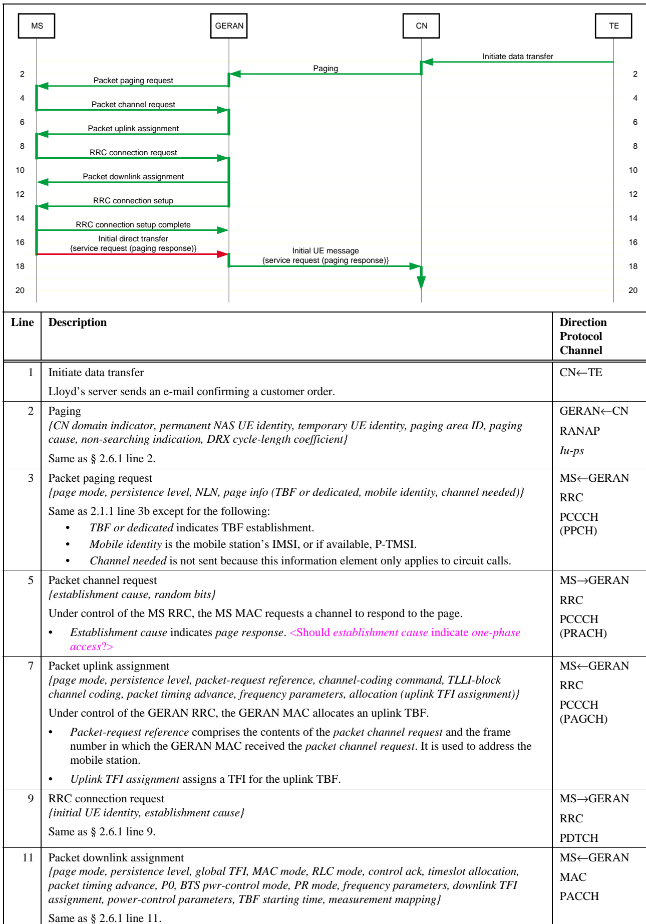
Figure 14: Incoming packet data transfer – RRC Idle, PCCCH, assign shared channel
