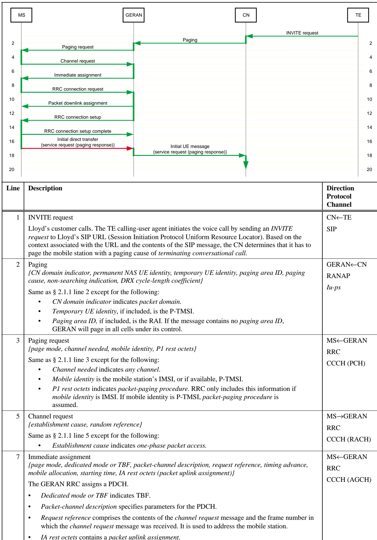
Figure 8: Incoming packet voice call – RRC-Idle, CCCH, assign shared channel
