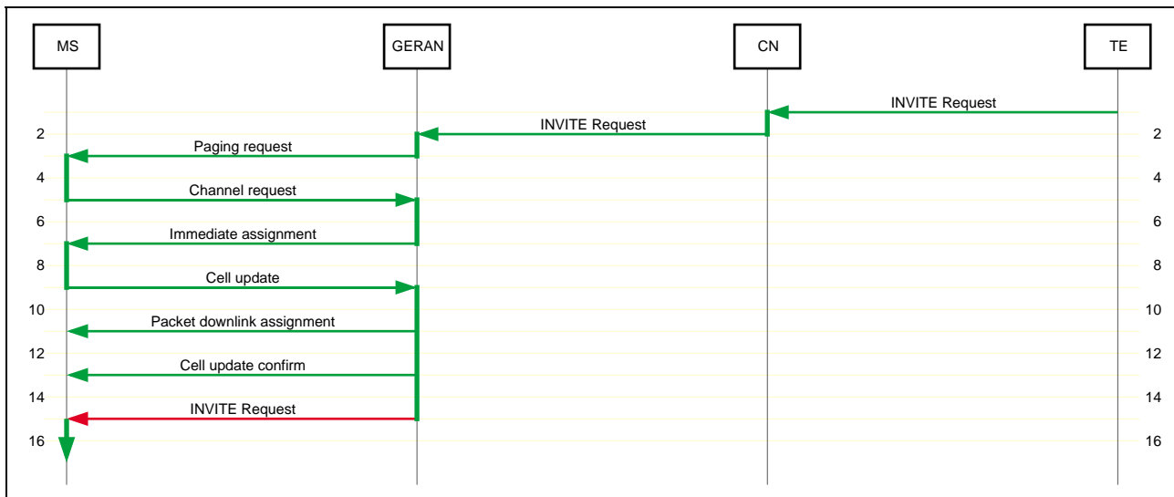
Figure 10: Incoming packet voice call – RRC-GRA_PCH, CCCH, assign shared channel
