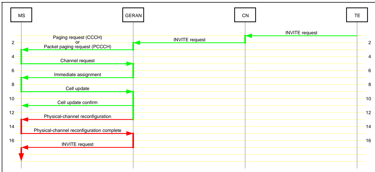
Figure 7: Incoming packet voice call – RRC-GRA_PCH, assign dedicated channel
