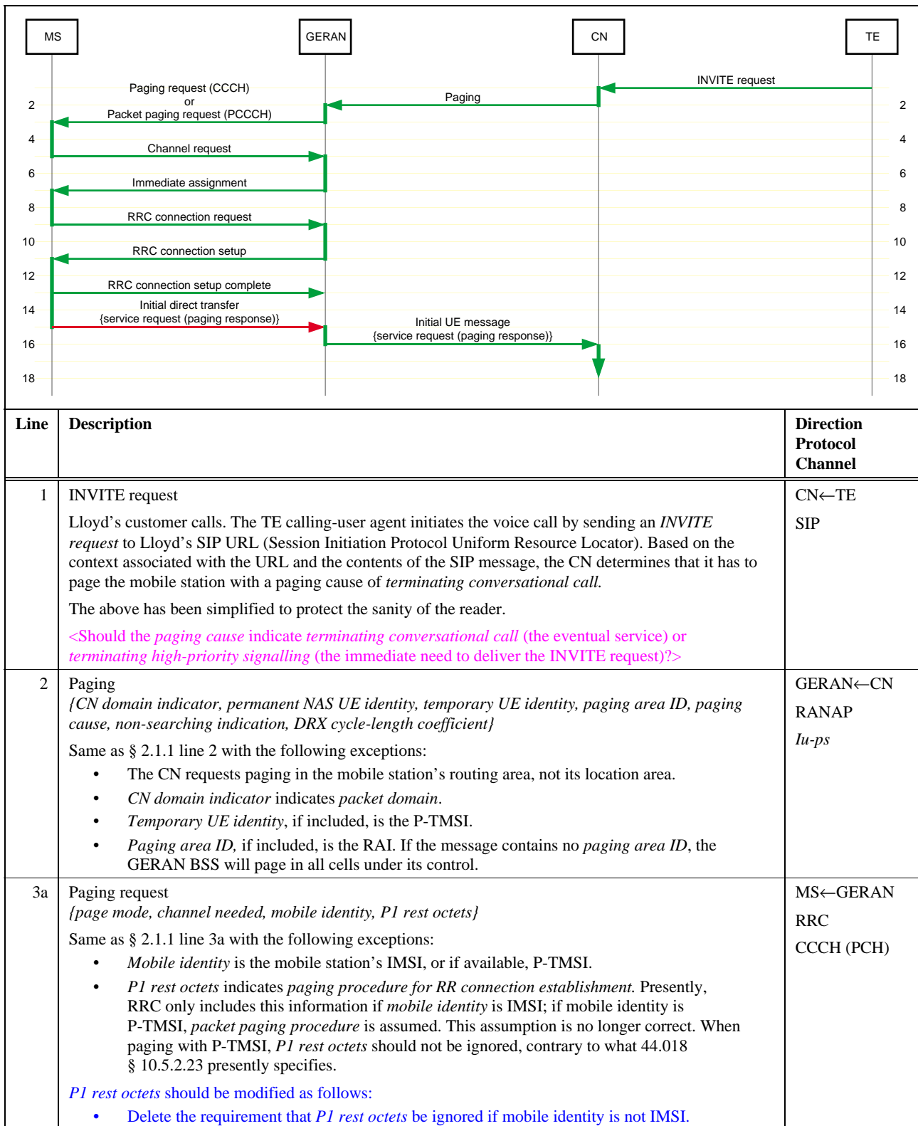
Figure 4: Incoming packet voice call – RRC-Idle, assign dedicated channel
