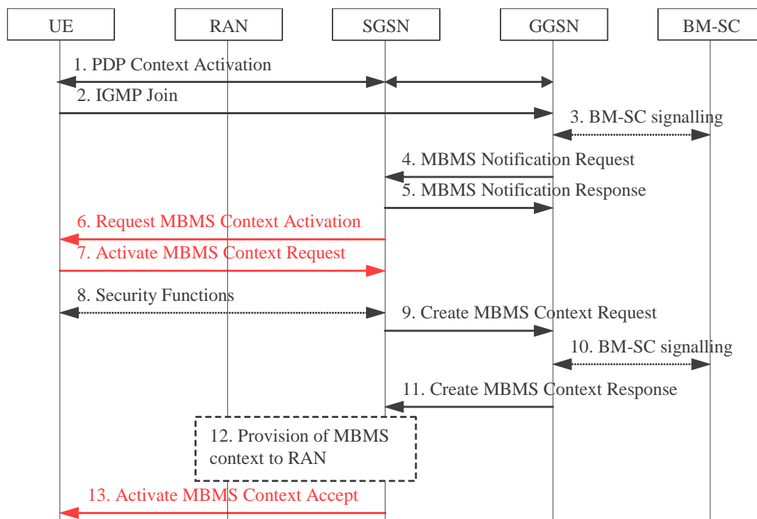
Figure 1. Activation of an MBMS Multicast service
