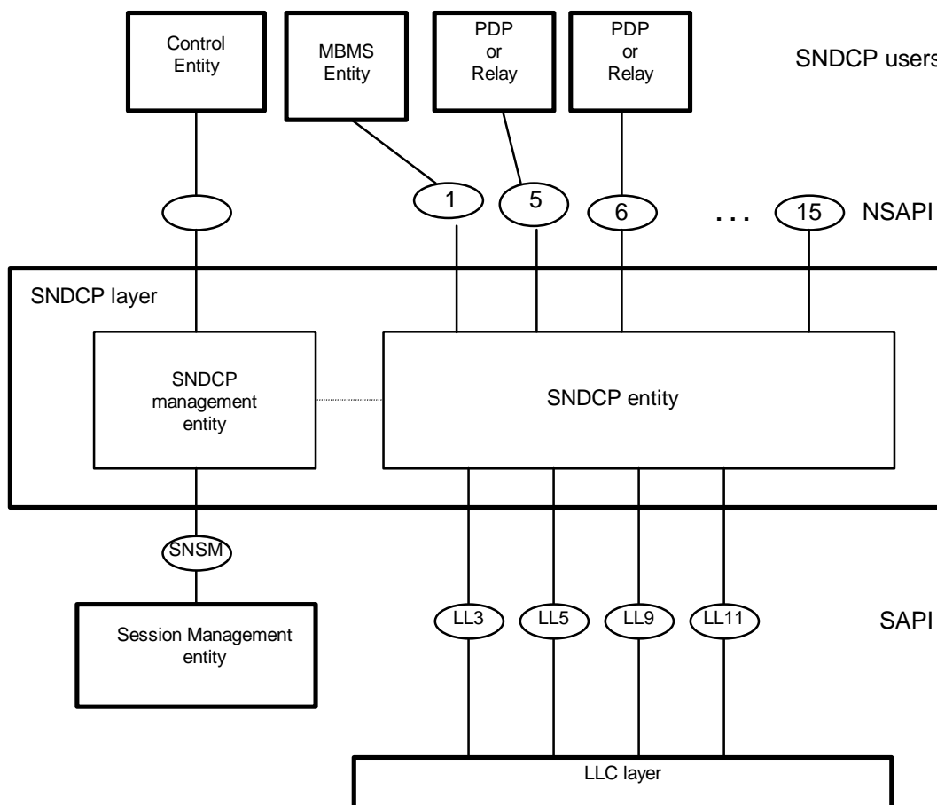
Figure 4: Service Access Points provided and used by SNDSCP
