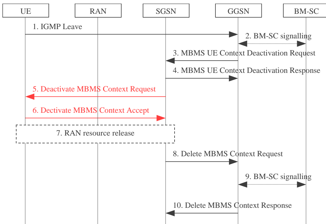
Figure 2: Deactivation of an MBMS Multicast service.
