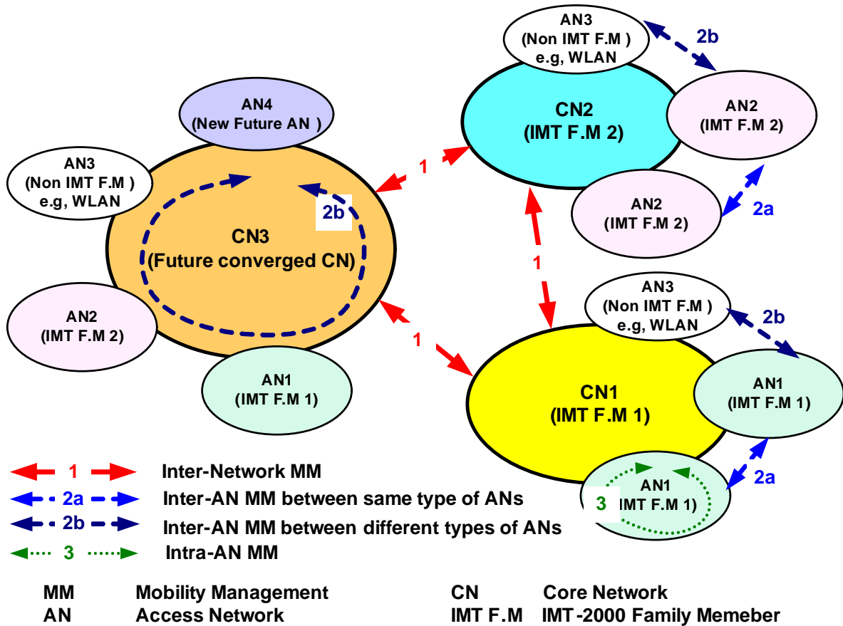
Figure 6.2 Interworking scenario for SBI2K network
