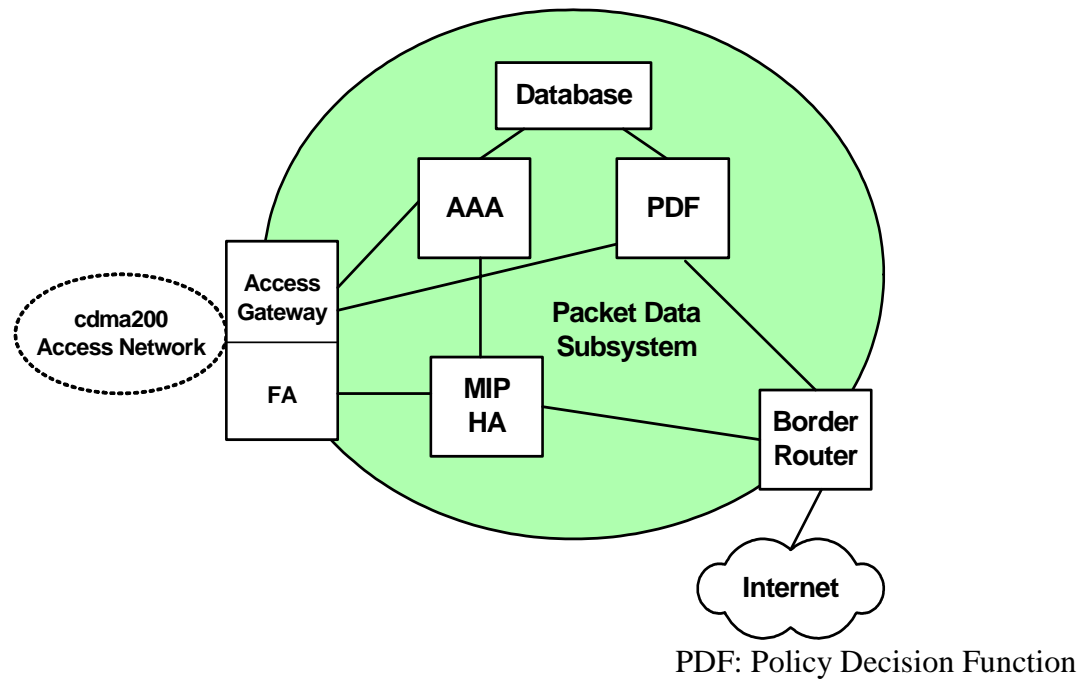
Figure 8.10 PDS of ANSI-41 evolved all-IP MMD Core Network
