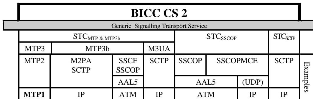
Figure: Signalling transport stacks for BICC call control protocol.
