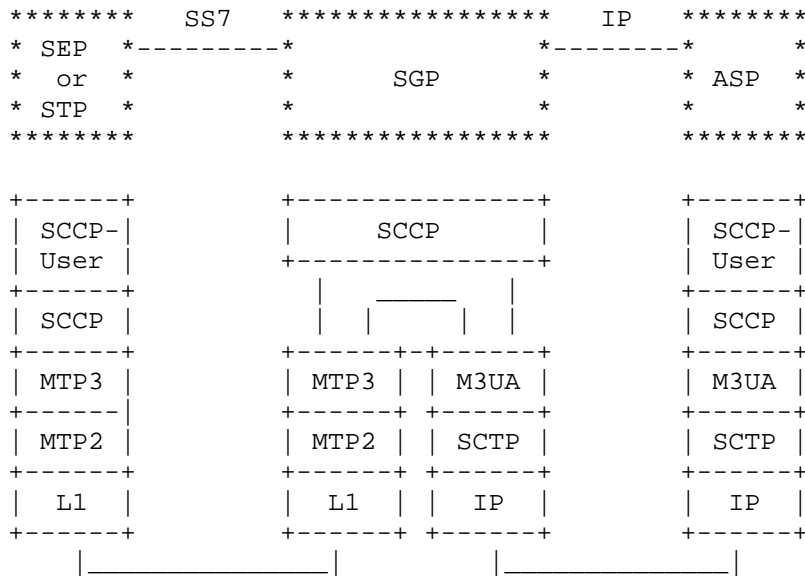
STP - SS7 Signalling Transfer Point
