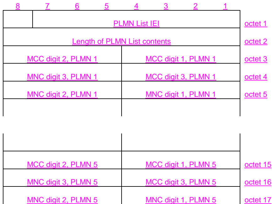
Figure 10.5.z/3GPP TS 24.008 PLMN List information element
