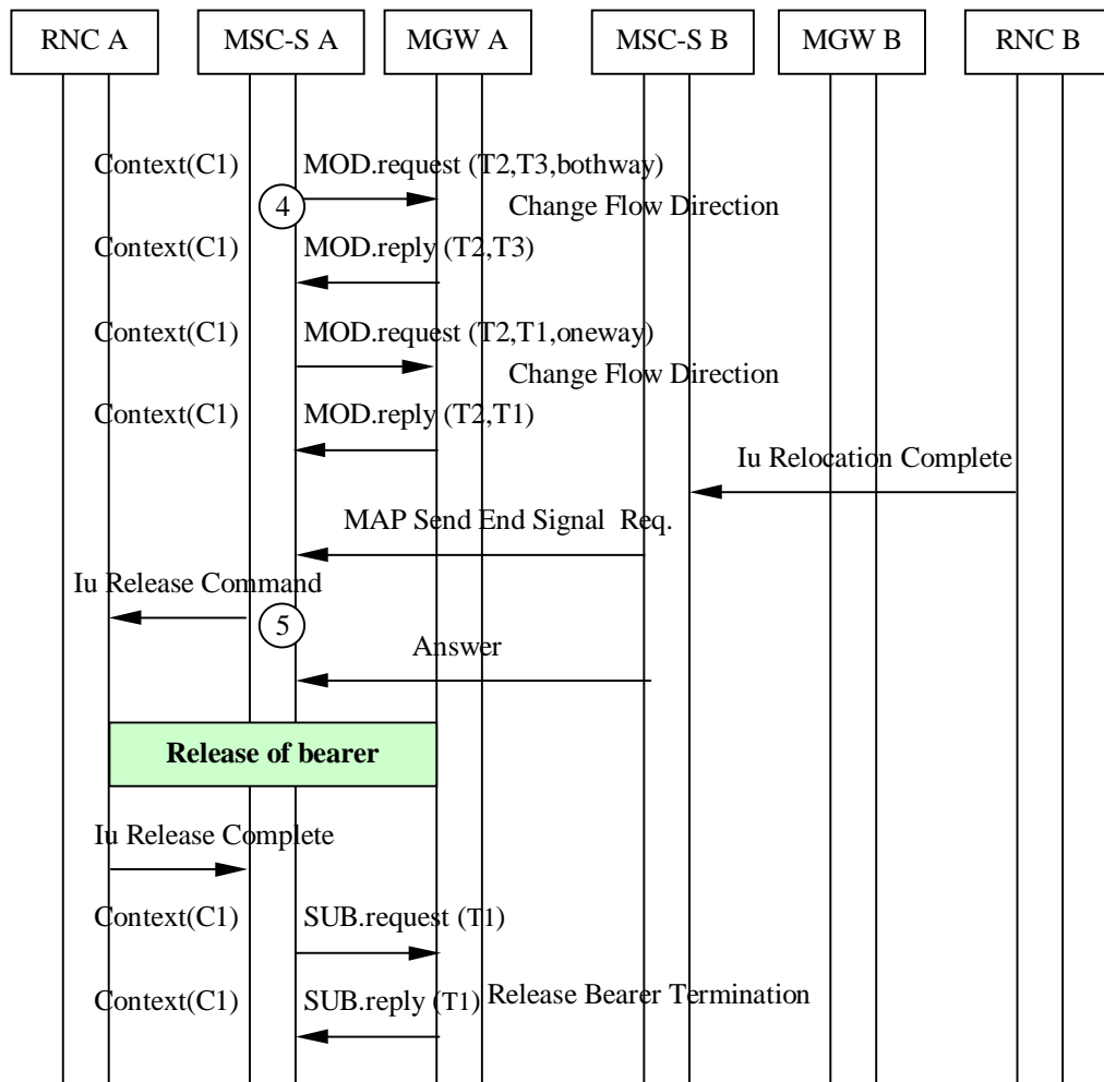
Figure 8.4/2 Basic Inter-MSR SRNS Relocation (message sequence chart)
