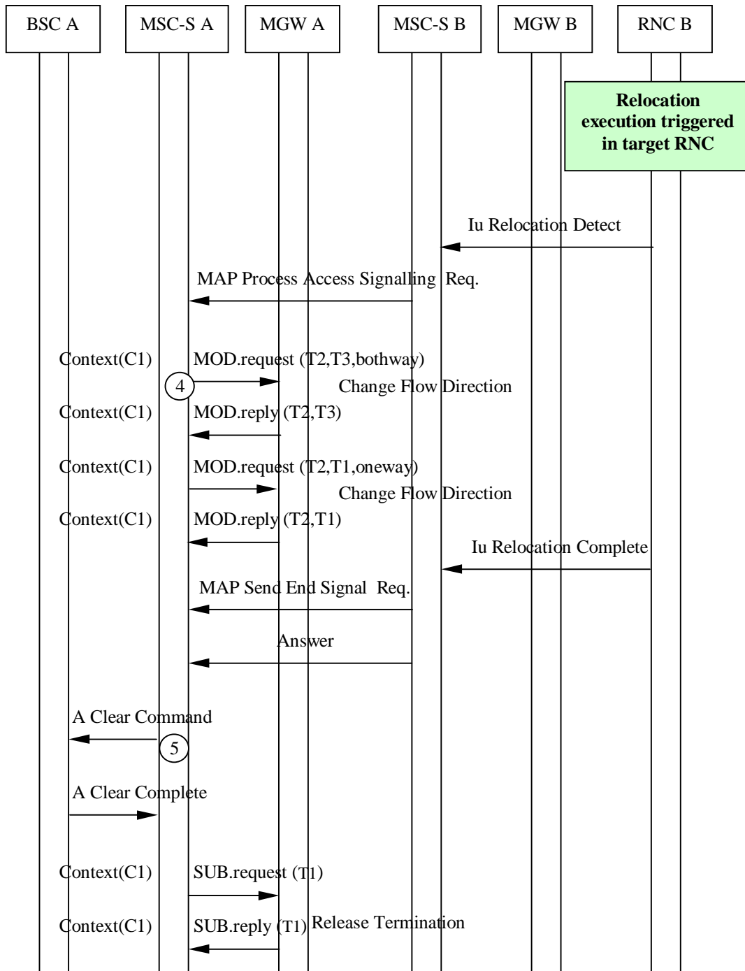
Figure 8.16/2 Basic Inter-MSM GSM to UMTS Handover (message sequence chart)
