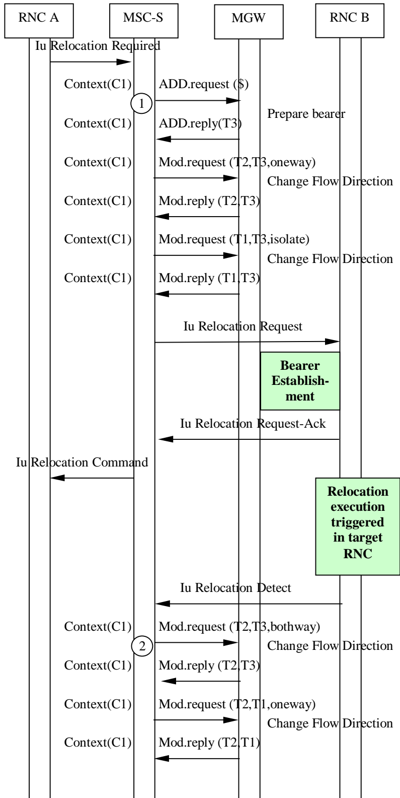
Figure 8.2/1 Intra-MSR SRNS Relocation (message sequence chart)
