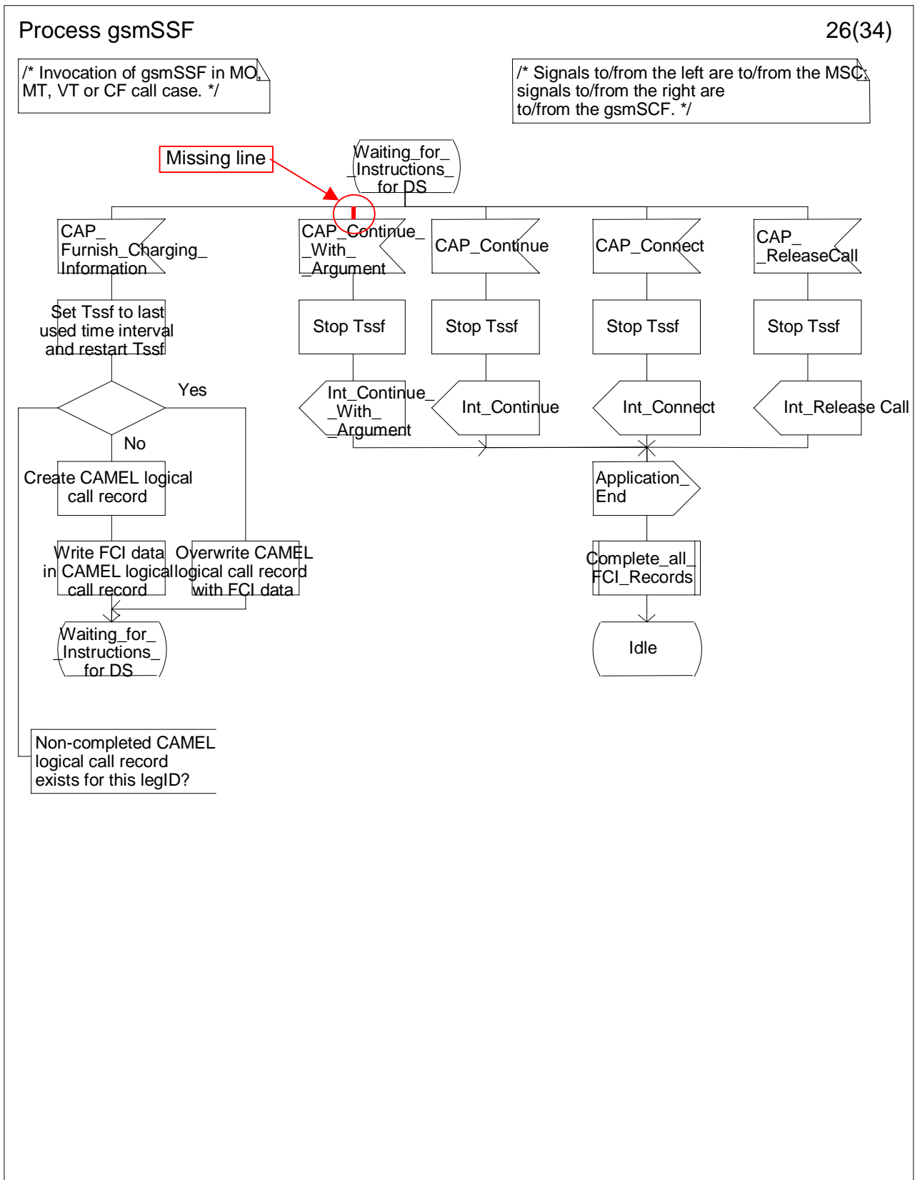
Figure 4.63z: Process gsmSSF (sheet 26)
