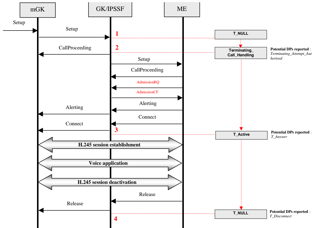
Figure 13: H.323 message flows and corresponding CAMEL T-BCSM for successful call establishment
