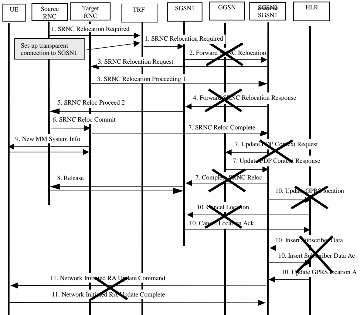
Figure 9: Information transfer for SRNS relocation update when changing SGSN area in a Turbo-Charged network
