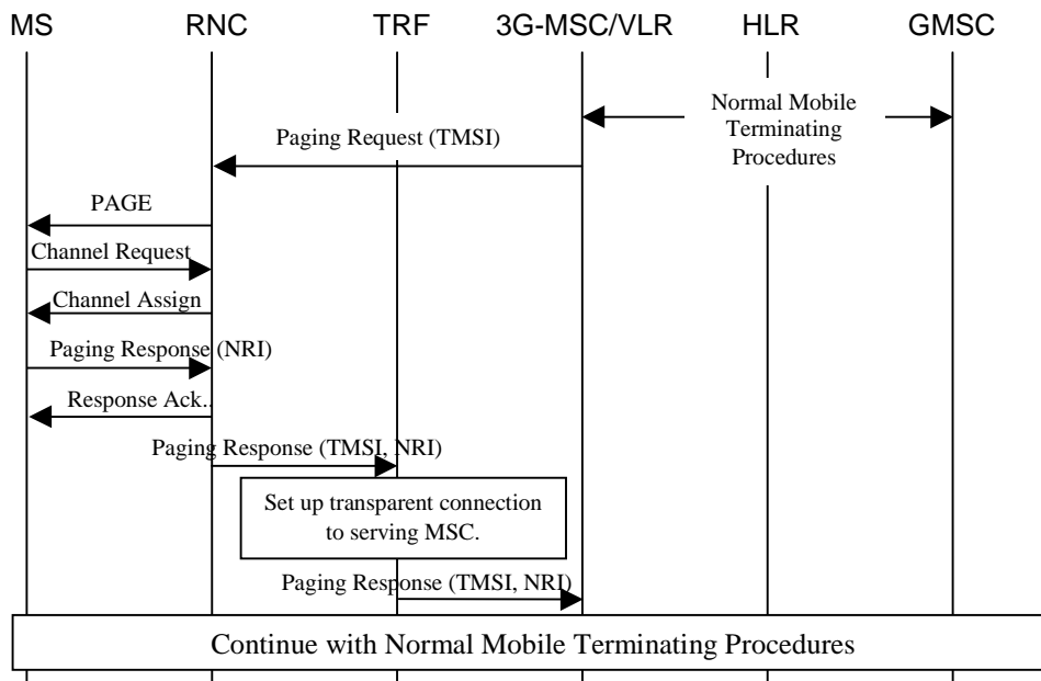
Figure 5: Mobile terminating call set-up procedure in a Turbo-Charged network.
