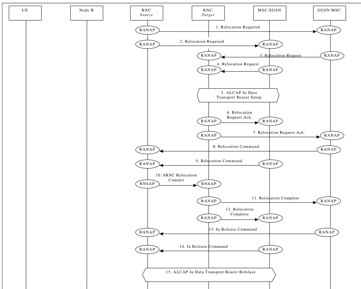
SRNS Relocation (UE connected to two CN nodes)
